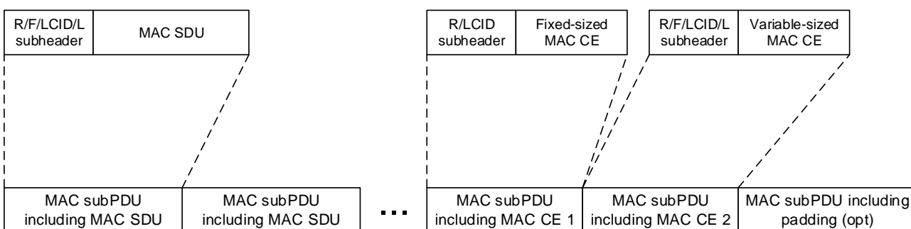
Figure 6.1.2-5: Example of a UL MAC PDU
