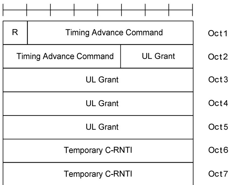
Figure 6.2.3-1: MAC RAR
