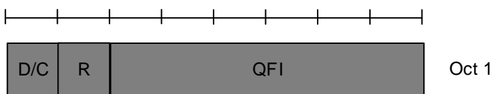
Figure 6.2.3-1: End-Marker Control PDU
