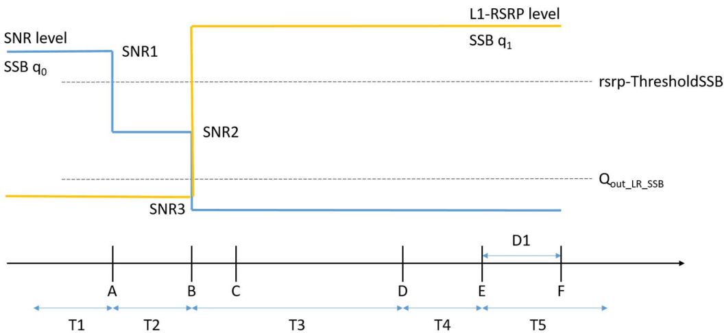
1: SNR and L1-RSRP for EN-DC FR2 SSB-based beam failure detection and link recovery in non-DRX
