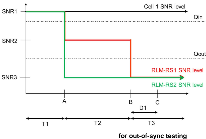
Figure 5.5.1.7.4-1: SNR variation for out-of-sync testing
