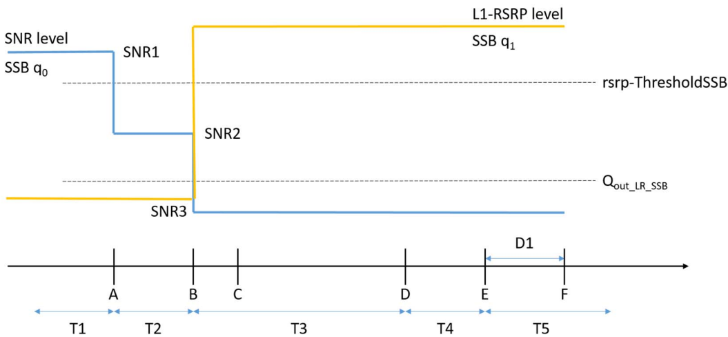
1: SNR and L1-RSRP for EN-DC FR2 SSB-based beam failure detection and link recovery in non-DRX
