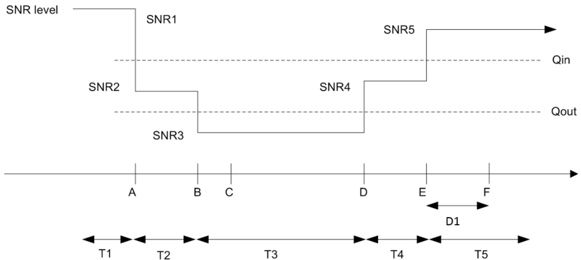
Figure 6.5.1.2.4-1 - SNR variation for in-sync testing
