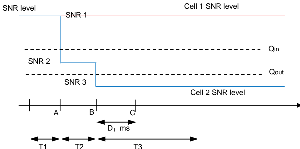
Figure 4.5.1.5.4-1: SNR variation for out-of-sync testing
