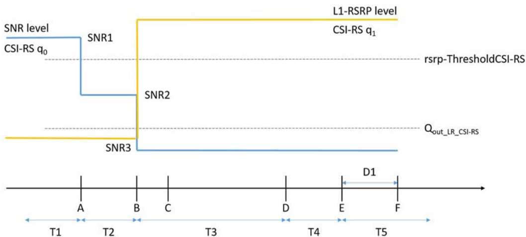
1: SNR and L1-RSRP variation for NR SA FR2 CSI-RS-based beam failure detection and link recovery in non-DRX
