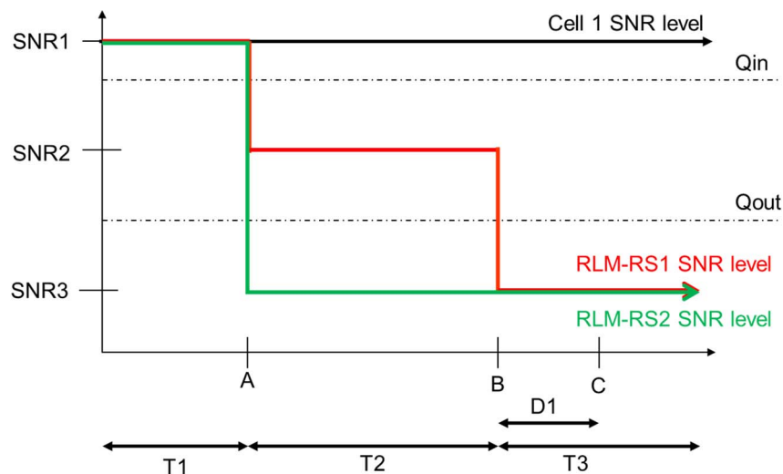
Figure 5.5.1.5.4-1: SNR variation for out-of-sync testing
