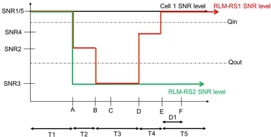
1: SNR variation for in-sync testing
