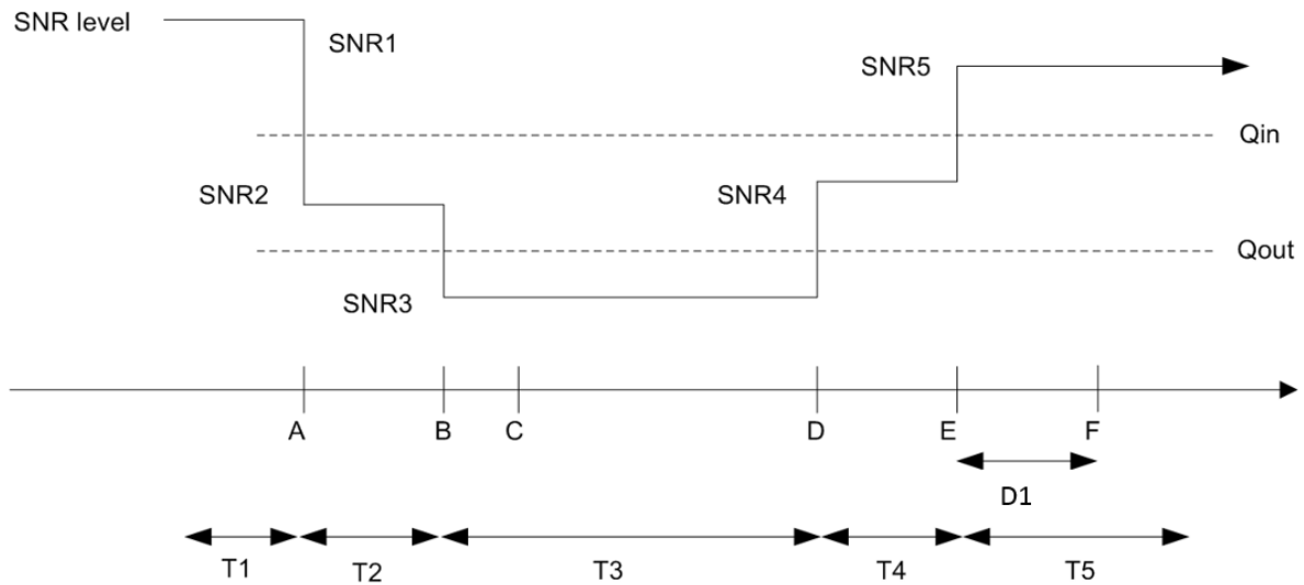
Figure 6.5.1.4.4-1 - SNR variation for in-sync testing
