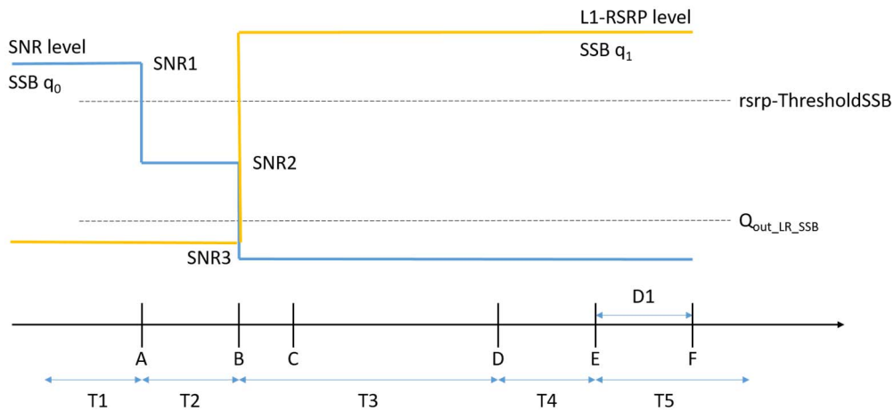
SNR and L1-RSRP variation for NR SA FR2 SSB-based beam failure detection and link recovery in non-DRX
