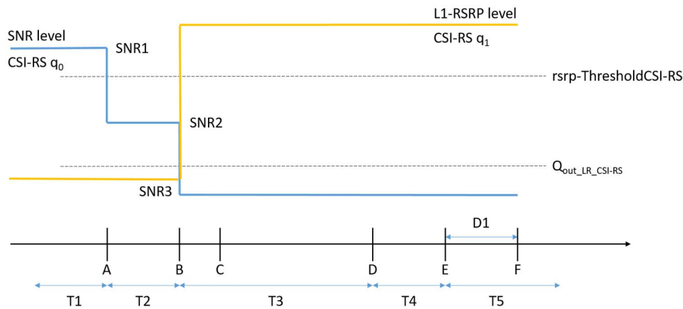
SNR and L1-RSRP variation for EN-DC FR2 CSI-RS-based beam failure detection and link recovery in non-DRX
