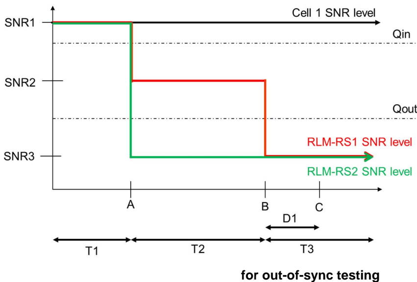
Figure 5.5.1.7.4-1: SNR variation
