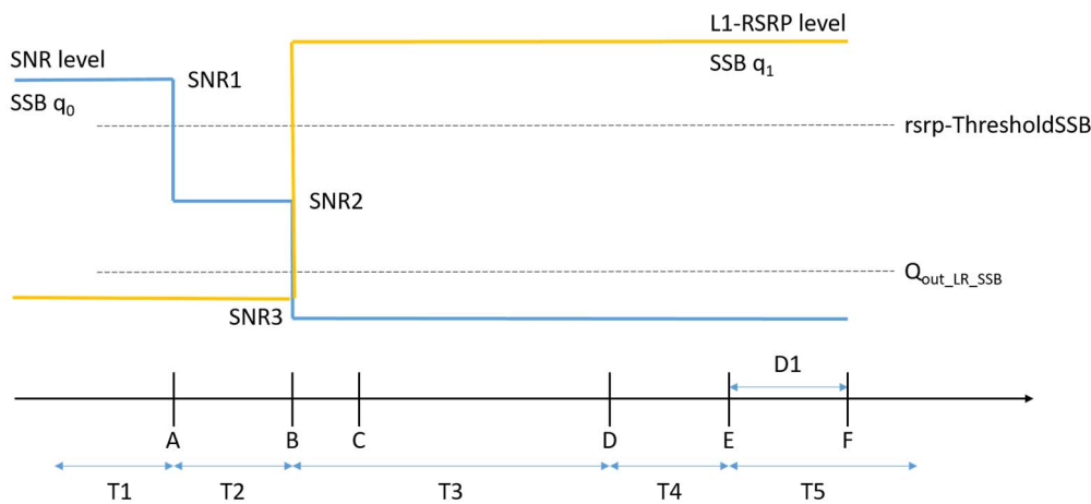
SNR and L1-RSRP variation for NR SA FR2 SSB-based beam failure detection and link recovery in non-DRX
