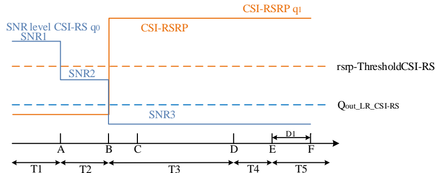
Figure 4.5.5.3.4-1: SNR and L1-RSRP variation for CSI-RS-based beam failure detection and link recovery testing in non-DRX mode
