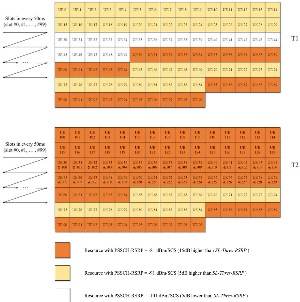
Figure 9.1.4.1.5-3: Power level variation of active sidelink UEs for NR SA FR1 L1 SL-RSRP measurement for resource re-evaluation
