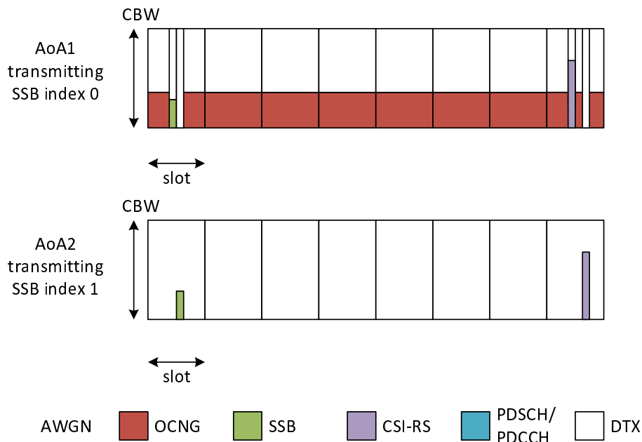
Figure 7.6.1.3.5-1: Time multiplexed downlink transmissions (Config 1 example) 7.6.1.4 NR SA FR2 event-triggered reporting with gap in DRX
