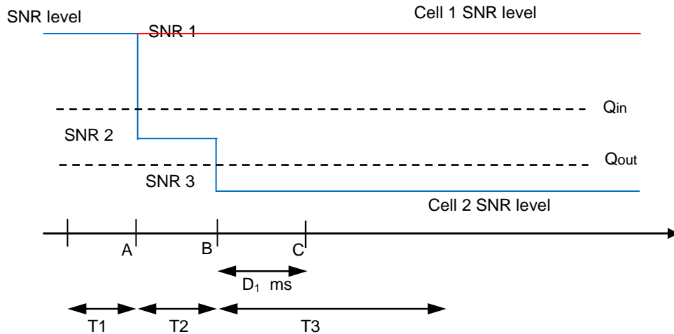
Figure 4.5.1.7.4-1: SNR variation for out-of-sync testing
