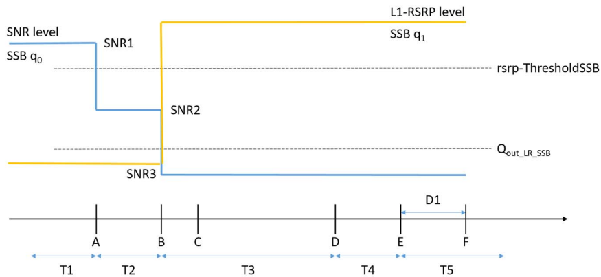
Figure 5.5.5.5.4-1: SNR and L1-RSRP variation for EN-DC FR2 scheduling available restriction during SSB-based beam failure detection and link recovery in non-DRX
