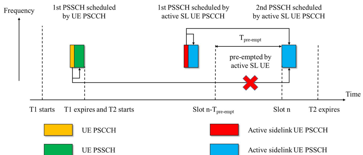
Figure 9.1.4.2.5-2: Power level variation of active sidelink UE for NR SA FR1 L1 SL-RSRP measurement for resource pre-emption
