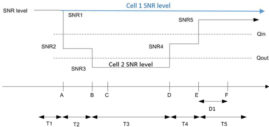
Figure 4.5.1.4.4-1 - SNR variation for in-sync testing
