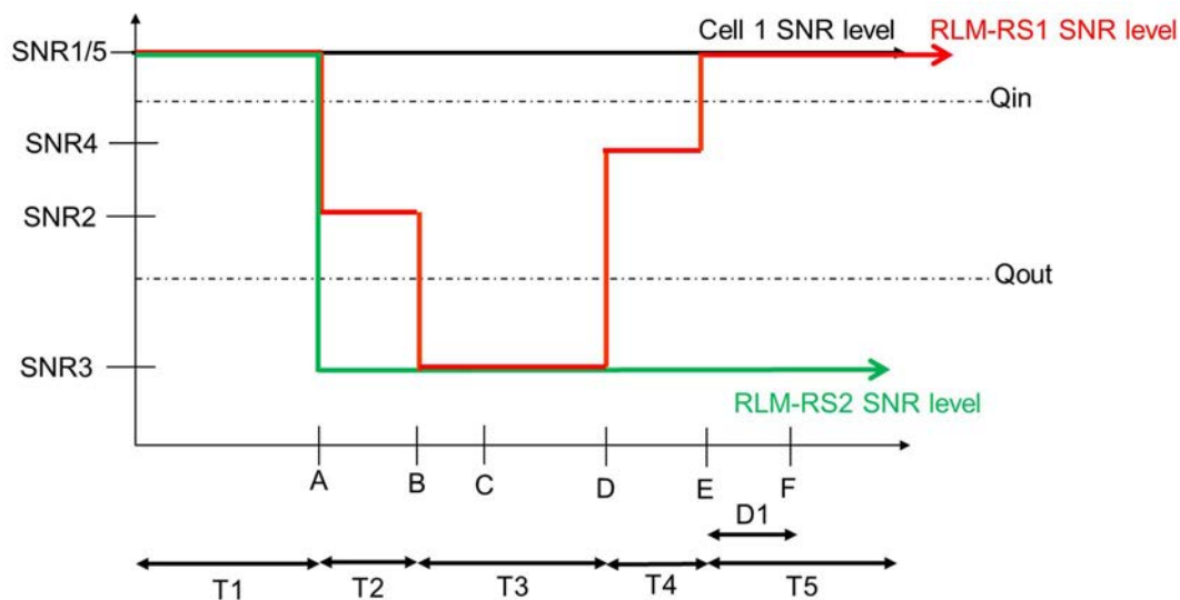
Figure 5.5.1.8.4-1: SNR variation for In-sync testing
