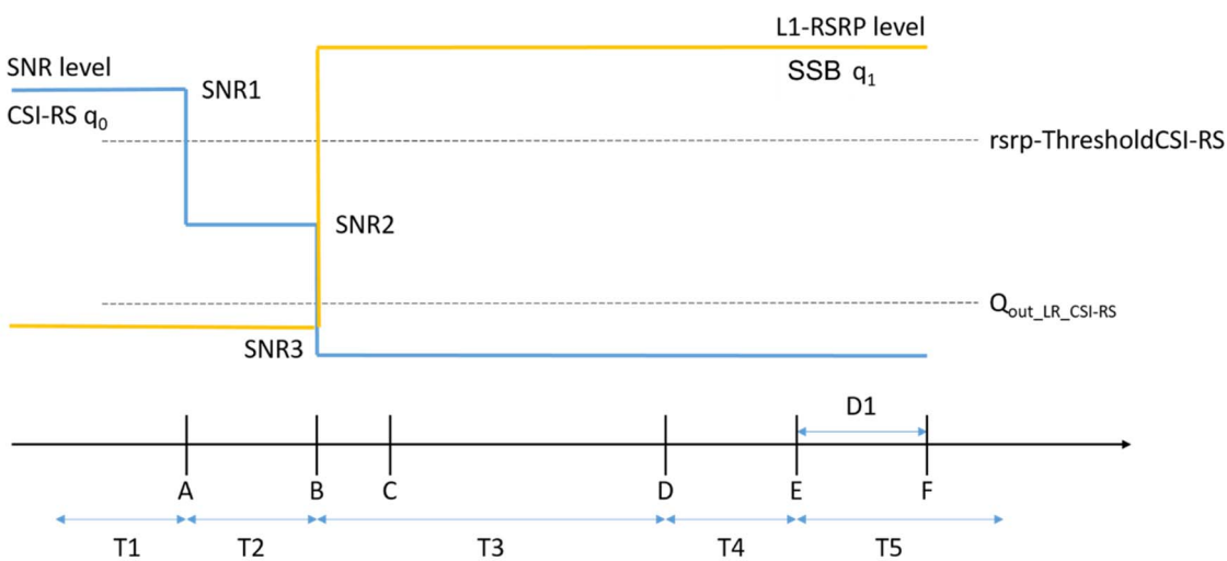
Figure 4.5.5.5.4-1: SNR and L1-RSRP variation for EN-DC FR1 CSI-RS-based beam failure detection and link recovery in DRX
