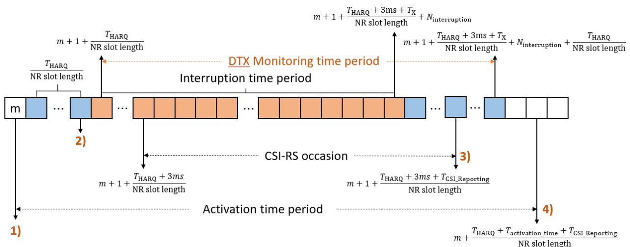
Figure 4.5.3.1.5-1: Procedure derivation for Activation
