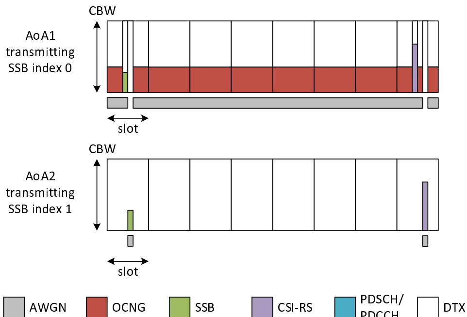
Figure 5.5.1.2.4-2: Time multiplexed downlink transmissions
