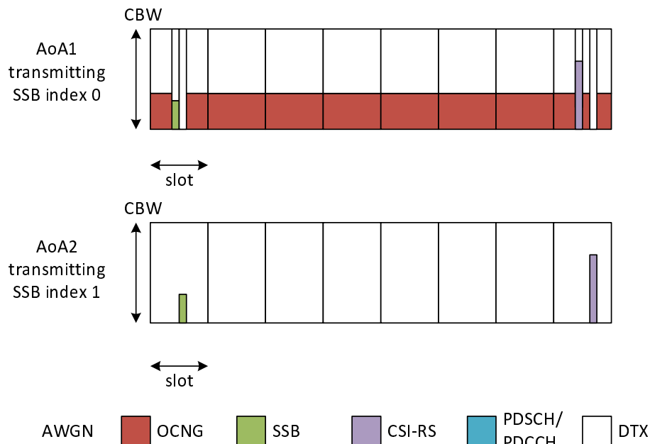
Figure 7.6.1.1.5-1: Time multiplexed downlink transmissions (Config 1 example)
