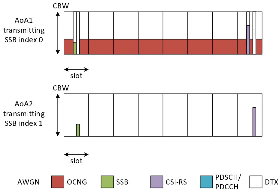
Figure 5.6.1.3.5-1: Time multiplexed downlink transmissions (Config 1,2 example)
