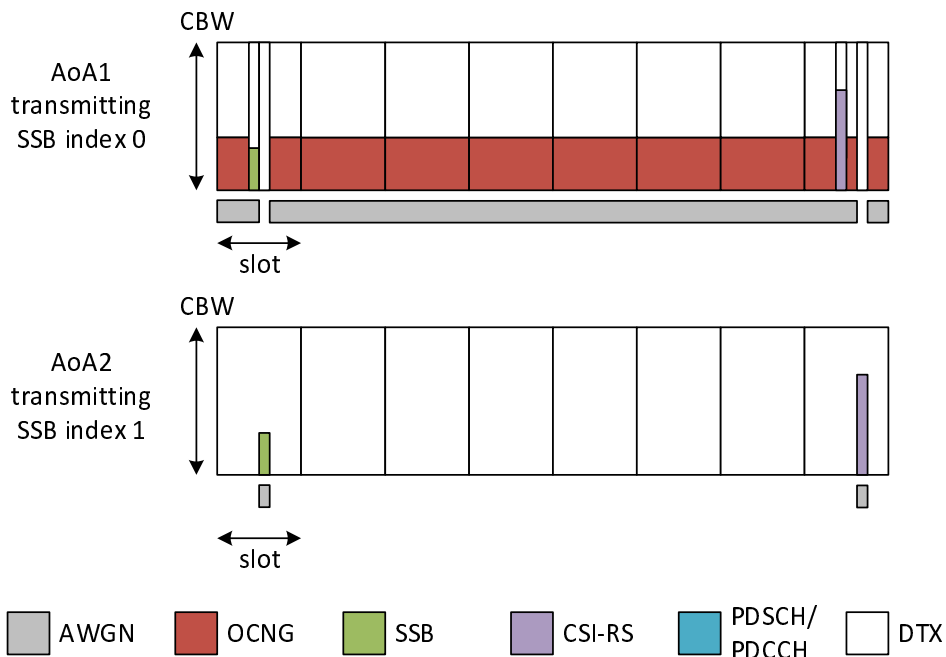
Figure 5.5.1.1.4-2: Time multiplexed downlink transmissions
