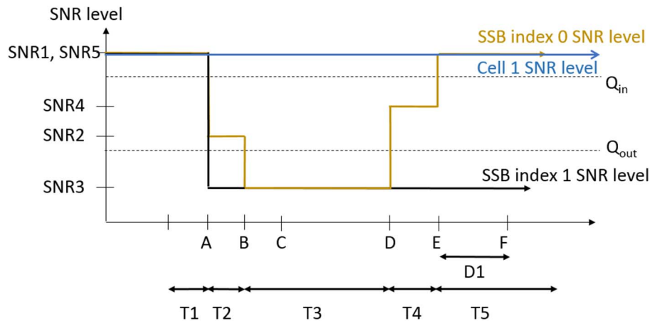
Figure 5.5.1.4.4-1: SNR variation for in-sync testing
