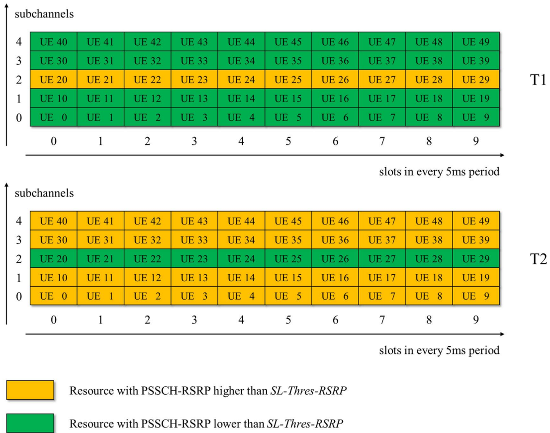
Figure 9.1.4.1.5-2: Power level variation of active sidelink UEs for NR SA FR1 L1 SL-RSRP measurement for autonomous resource selection/reselection
