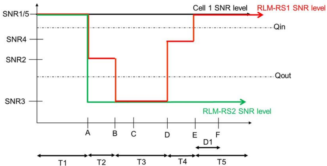
Figure 5.5.1.6.4-1: SNR variation for in-sync testing
