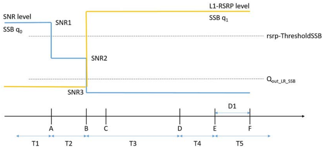
Figure 5.5.5.1.4-1: SNR and L1-RSRP for EN-DC FR2 SSB-based beam failure detection and link recovery in non-DRX
