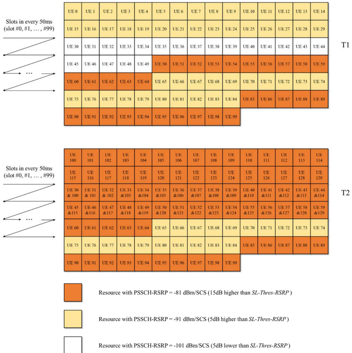
Figure 9.1.4.3.5-3: Power level variation of active sidelink UEs for NR SA FR1 L1 SL-RSRP measurement for resource re-evaluation
