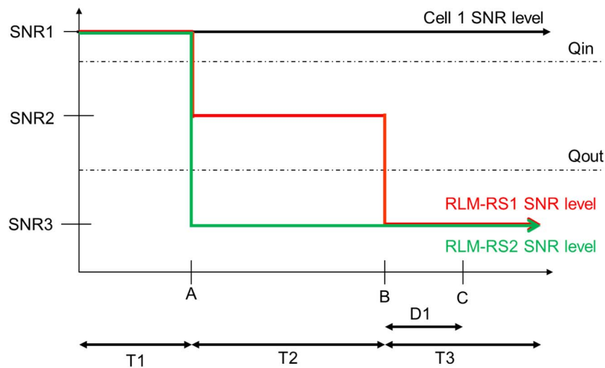
Figure 5.5.1.7.4-1: SNR variation for out-of-sync testing
