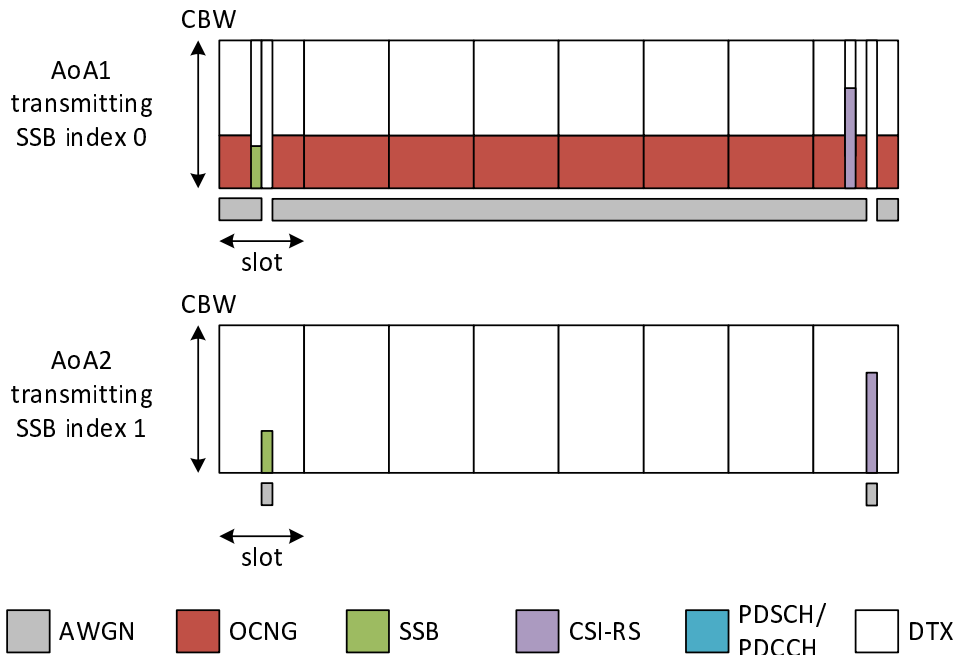
Figure 7.5.1.9.4-1: Time multiplexed downlink transmissions
