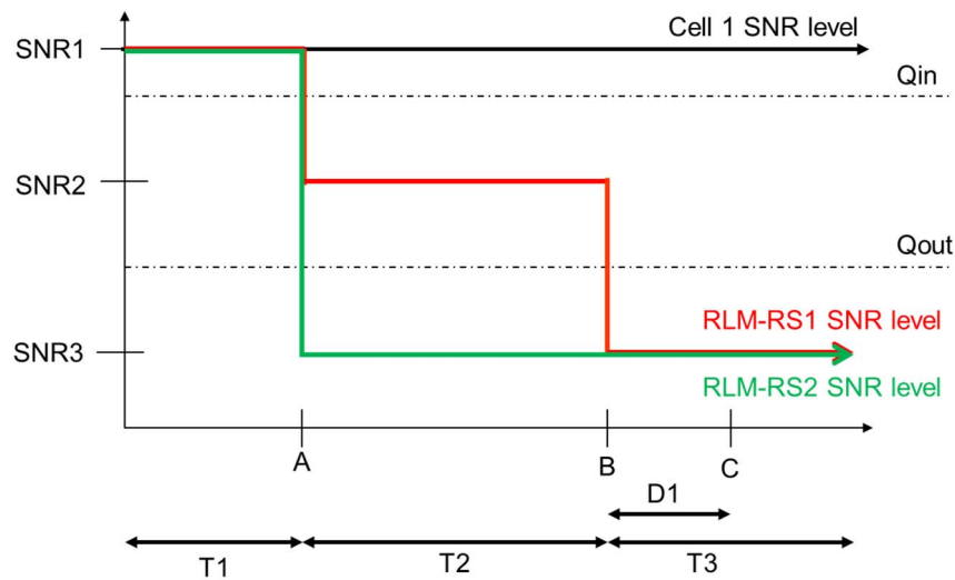
Figure 5.5.1.5.4-1: SNR variation for out-of-sync testing
