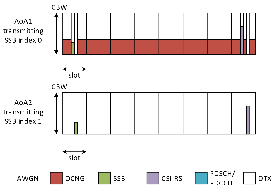
Figure 5.6.1.1.5-1: Time multiplexed downlink transmissions (Config 1,2 example)
