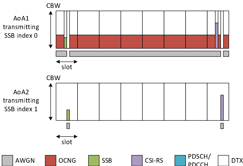
Figure 5.5.1.9.4-1: Time multiplexed downlink transmissions
