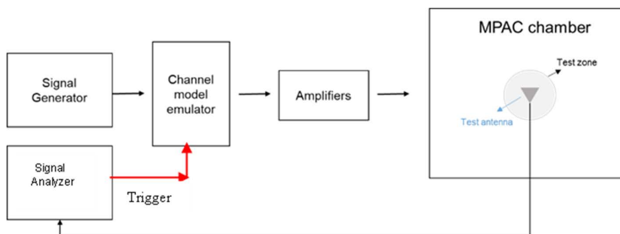
Figure I.3.3-2: Setup for Doppler measurements based on time domain technique
