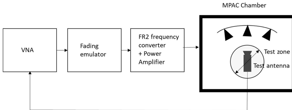
Figure I.3.2-1: Setup for PDP measurements (FR2)
