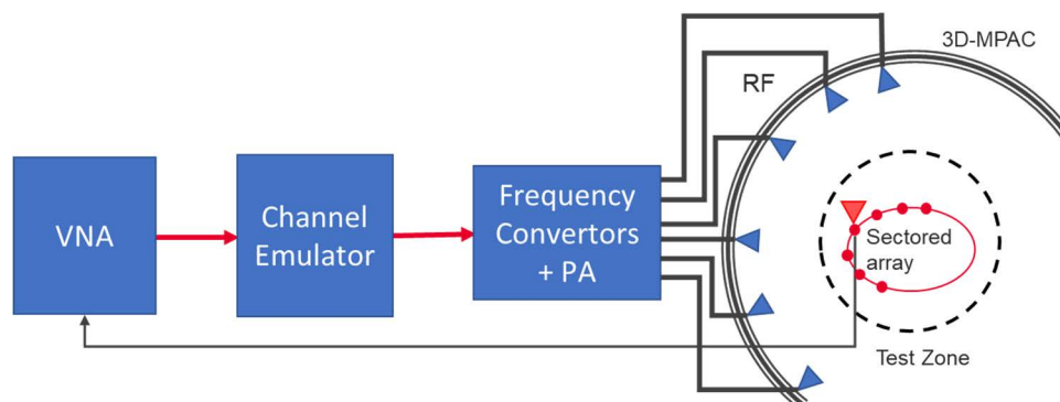
Figure I.3.4-2: Setup for FR2 PSP validation measurements
