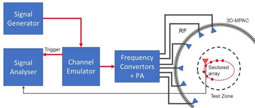
Figure I.3.4-3: Setup for FR2 PSP validation measurements based on time domain
