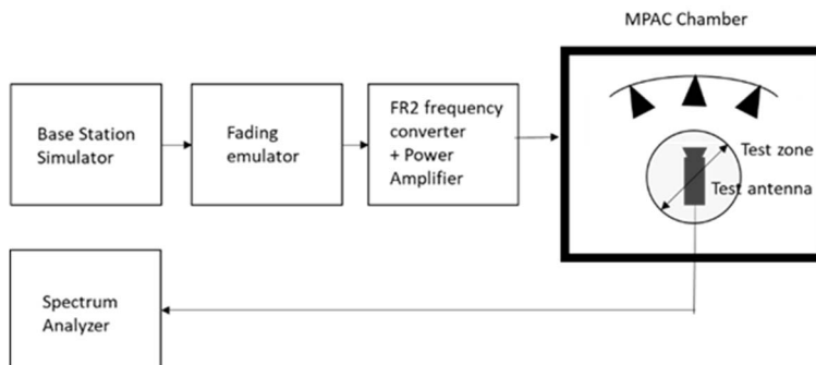
Figure I.3.6-1: Setup for FR2 power validation measurements
