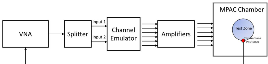
Figure C.3.4-2: Configuration for spatial correlation validation (CDL-C UMi)
