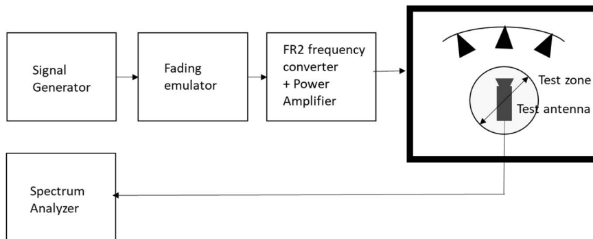
Figure I.3.3-1: Setup for FR2 Doppler measurements
