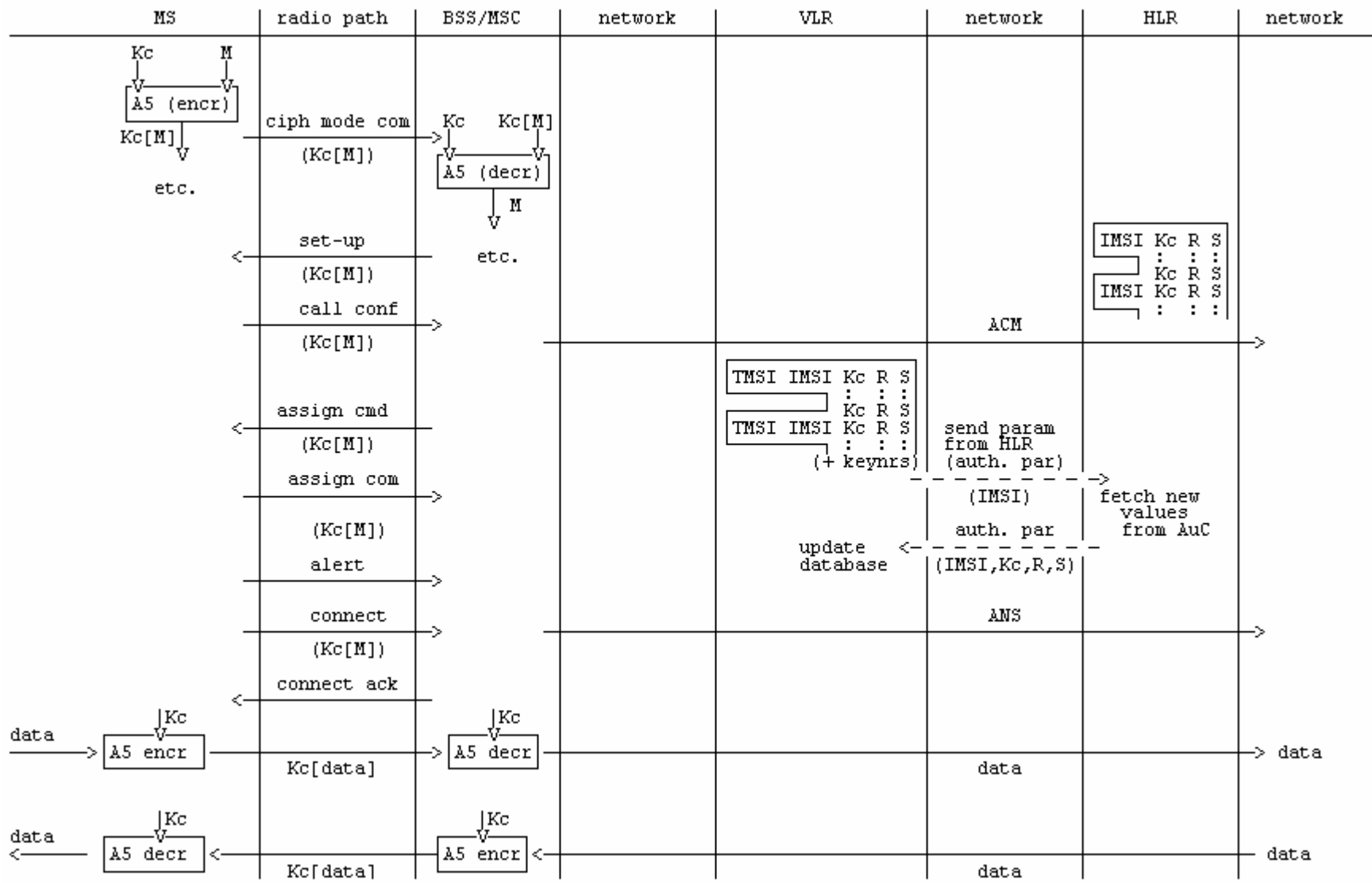
Scheme 7 (concluded)
