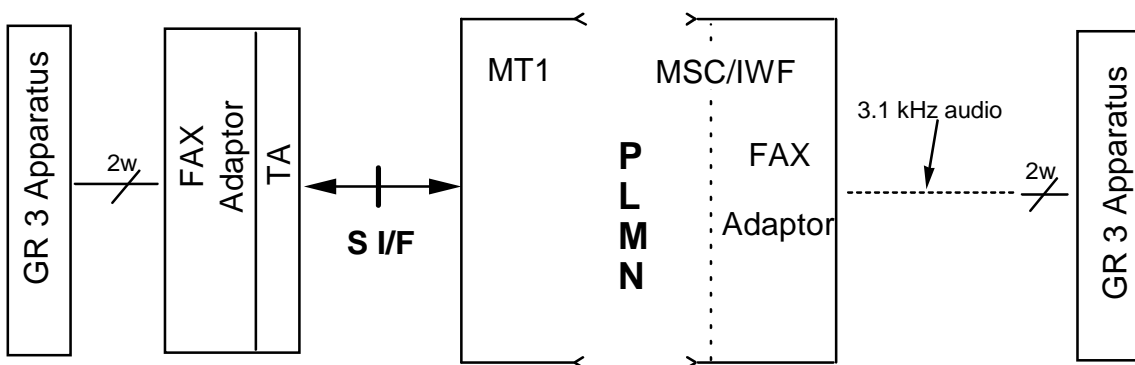
Figure 4b/43.045: Optional Teleservice connection (F.F.S)
