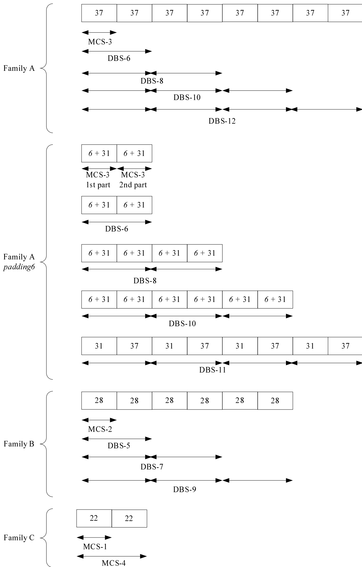
Figure 18b: General description of the Modulation and Coding Schemes for EGPRS2-B in the downlink
