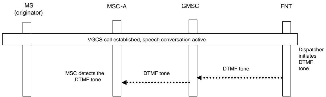
Figure 7d: Signalling required for communication of DTMF digit entry by an entitled fixed line dispatcher in case DTMF tone is used.
