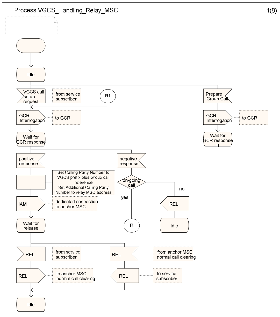
Figure 10: The VGCS handling process in the relay MSC (sheet 1 of 8)
