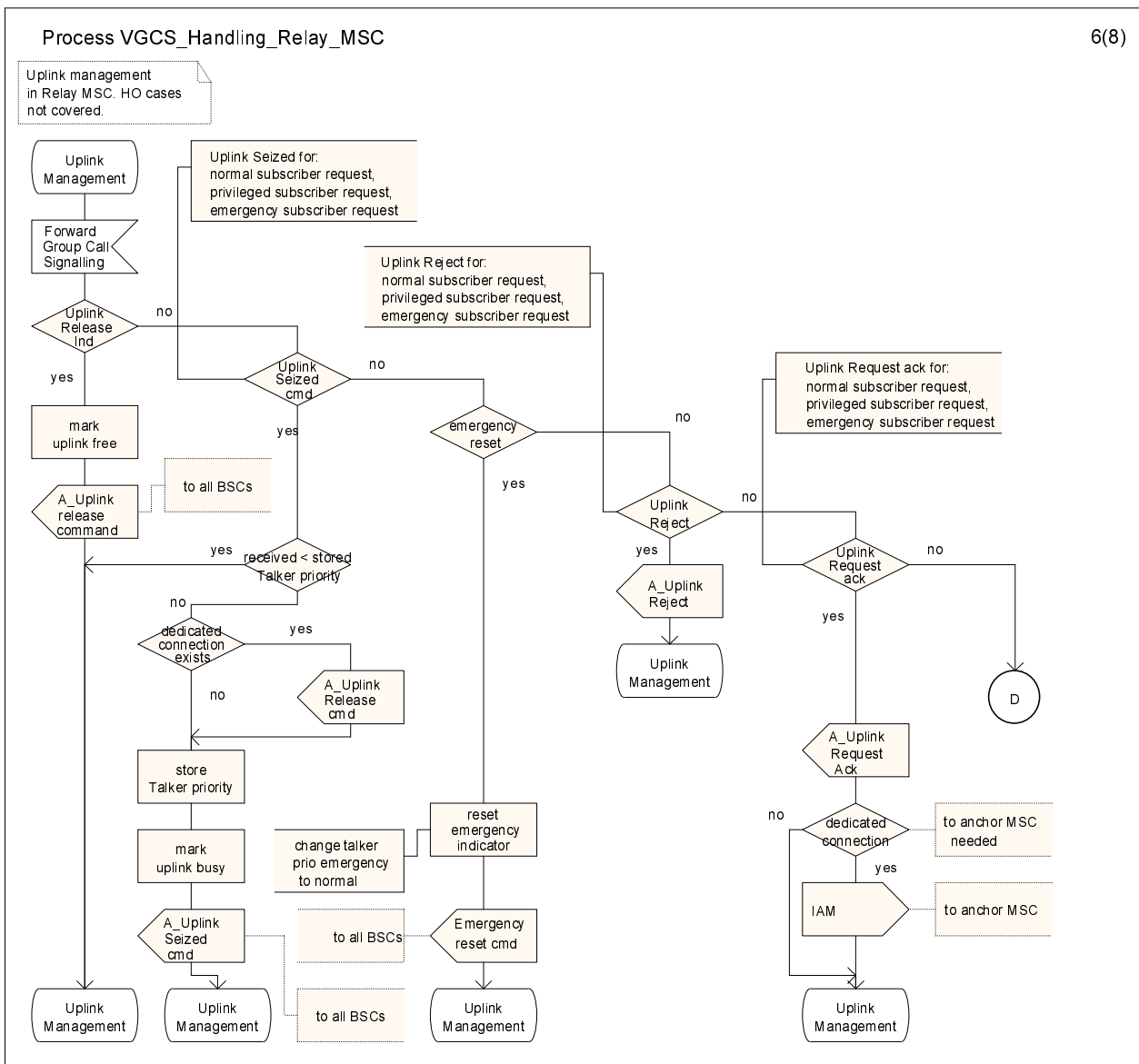
Figure 10: The VGCS handling process in the relay MSC (sheet 6 of 8)
