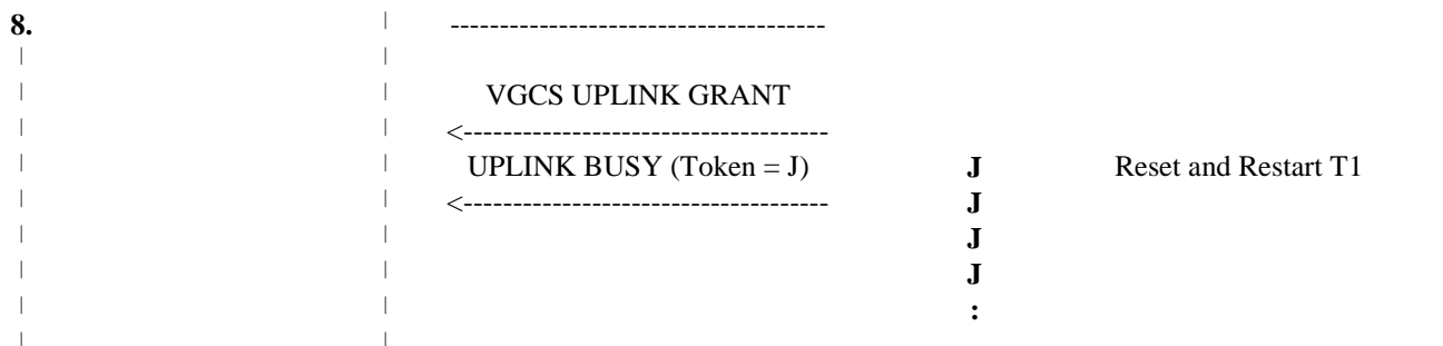
Figure 7e: Validation of Priority Uplink Requests for ciphered group calls
