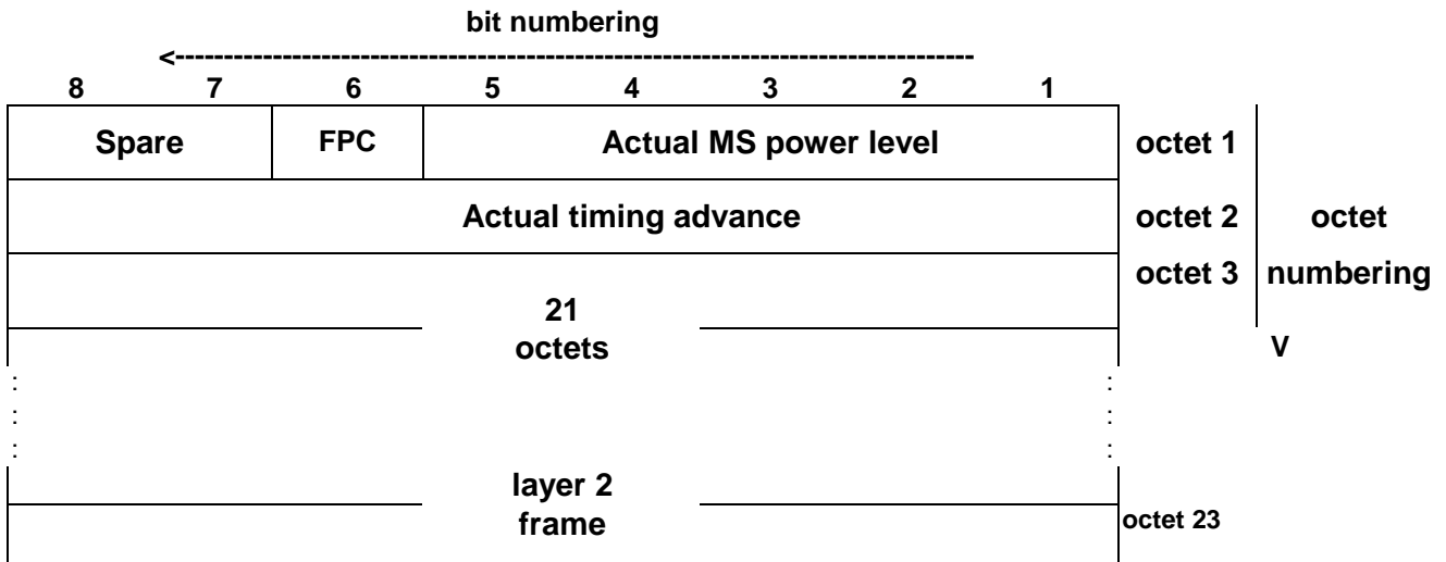
Figure 7.2: SACCH uplink block format
