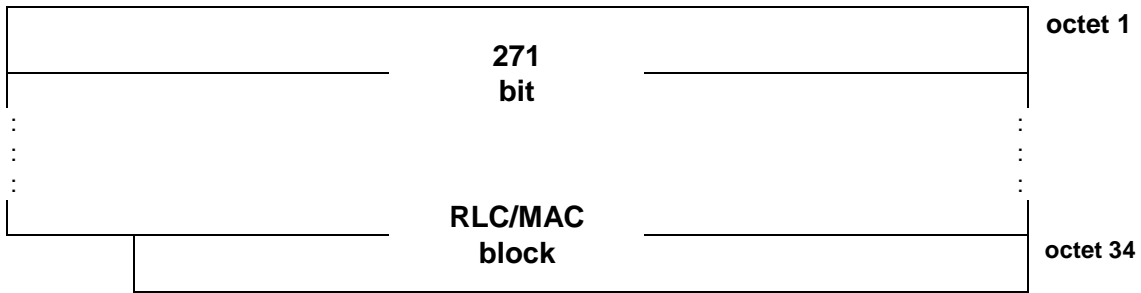
Figure 7.6: PDTCH block type 2 (CS-2) format
