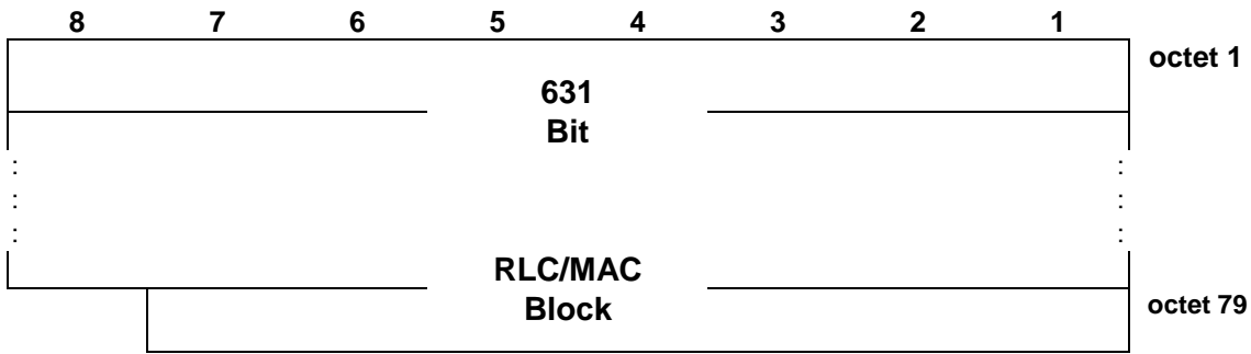
Figure 7.6.10.1: PDTCH block type 10 (MCS-6) uplink format
