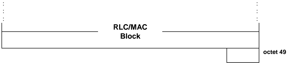
Figure 7.6.8: PDTCH block type 8 (MCS-4) format
