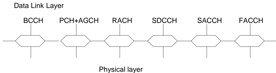
Figure 3.1.b: SAPs between the physical layer and the data link layer when the MS is operating in A/Gb mode
