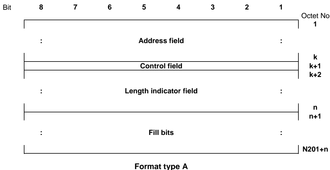
Figure 1 (sheet 1 of 3): General frame formats
