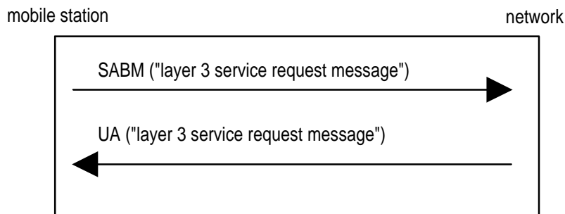
Figure 3.1.5.1/3GPP TS 44.018: Service request and contention resolution
