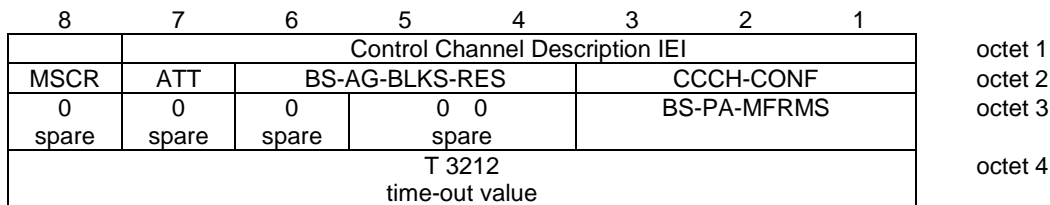
Figure 10.5.2.11.1/3GPP TS 44.018: Control Channel Description information element
