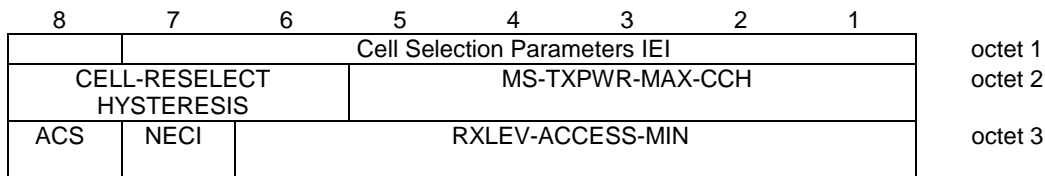
Figure 10.5.2.4.1/3GPP TS 44.018: Cell Selection Parameters information element
