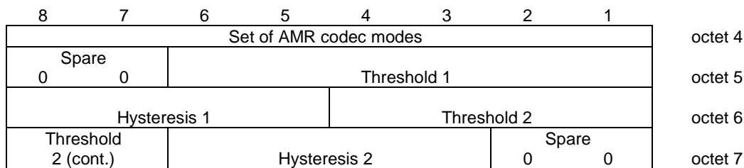
Figure 10.5.2.21aa.4/3GPP TS 44.018: Parameters for multirate speech field for the Multirate speech versions 1 & 3 when a set of three codec modes is chosen
