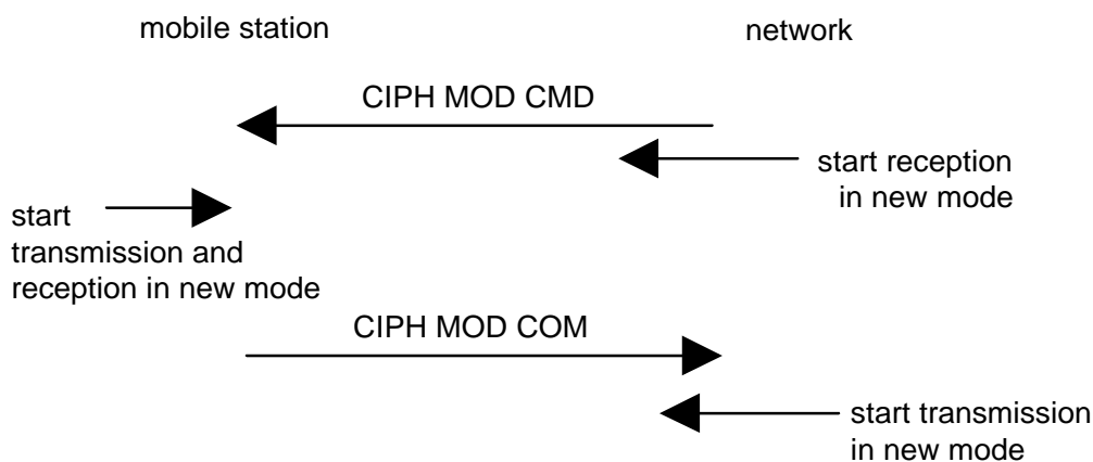
Figure 3.4.7.2.1/3GPP TS 44.018: Ciphering mode setting sequence
