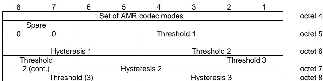
Figure 10.5.2.21aa.5/3GPP TS 44.018: Parameters for multirate speech field for the Multirate speech versions 1 & 3 when a set of four modes is chosen
