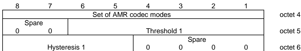
Figure 10.5.2.21aa.3/3GPP TS 04: Parameters for multirate speech field for the Multirate speech versions 1 & 3 when a set with two codec modes is chosen
