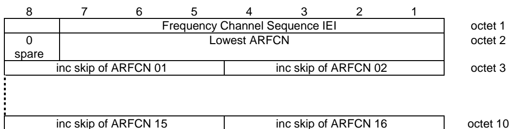
Figure 10.5.2.12.1/3GPP TS 44.018: Frequency Channel Sequence information element
