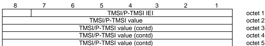
Figure 10.5.2.42.1/3GPP TS 44.018: TMSI/P-TMSI information element
