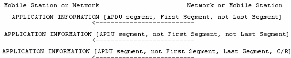
Figure 3.4.21.3.2.1/3GPP TS 44.018: Application Information Transfer with segmentation
