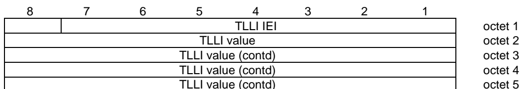
Figure 10.5.2.41a.1/3GPP TS 44.018: TLLI information element
