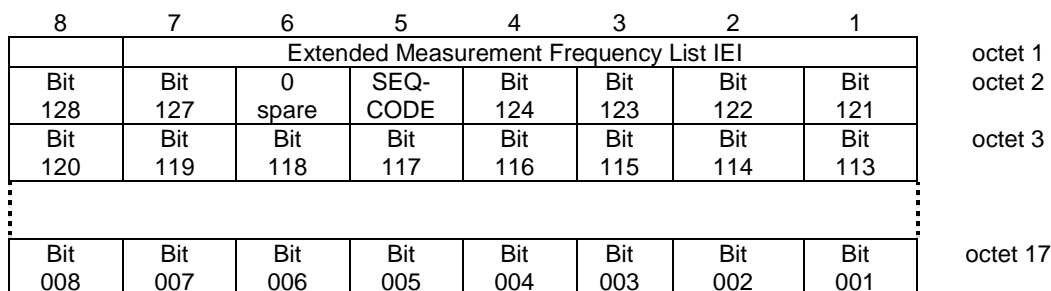
Figure 10.5.2.46.1/3GPP TS 44.018: Extended Measurement Frequency List information element
