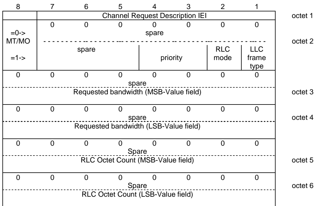
Figure 10.5.2.8a.1/3GPP TS 44.018: Channel Request Description information element
