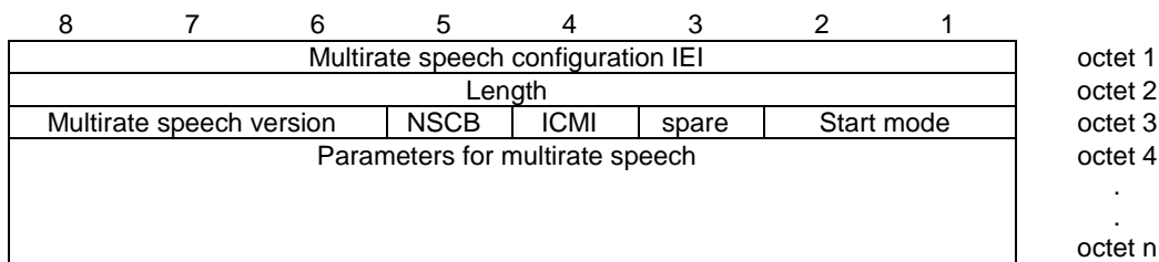
Figure 10.5.2.21aa.1/3GPP TS 44.018: MultiRate configuration information element
