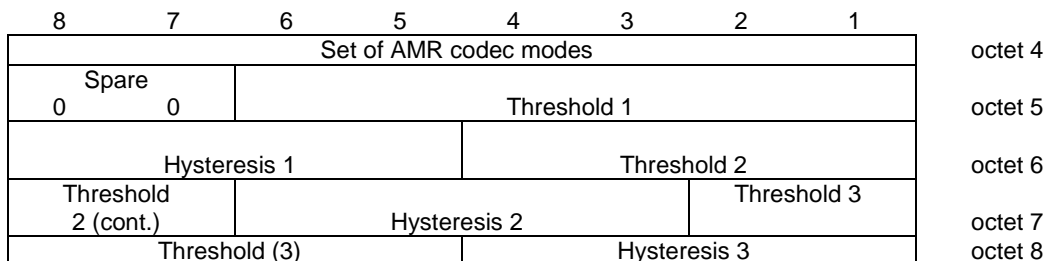
Figure 10.5.2.21aa.5/3GPP TS 44.018: Parameters for multirate speech field for the Multirate speech versions 1 & 2 when a set of four modes is chosen
