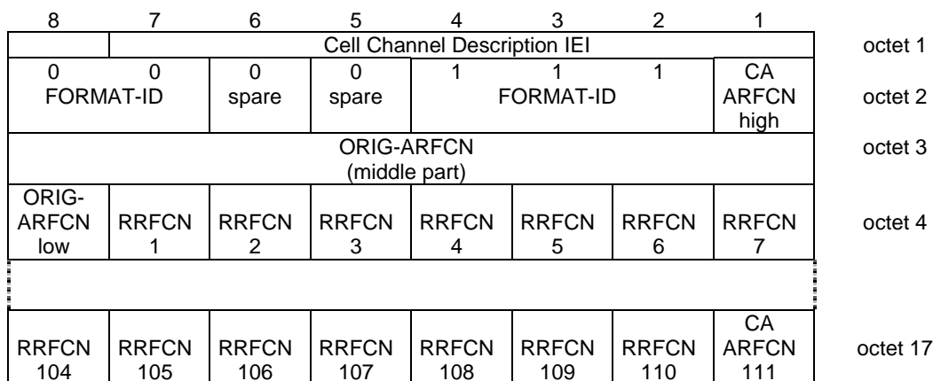
Figure 10.5.2.1b.7.1/3GPP TS 44.018: Cell Channel Description information element, variable bit map format
