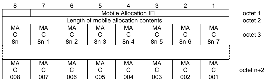
Figure 10.5.2.21.1/3GPP TS 44.018: Mobile Allocation information element
