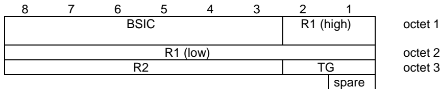
Figure 9.1.30b.1/3GPP TS 44.018: COMPACT Frame synchronization information element
