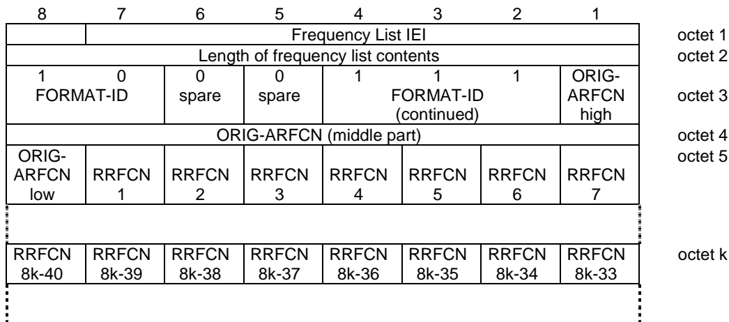
Figure 10.5.2.13.7.1/3GPP TS 44.018: Frequency List information element, variable bit map format
