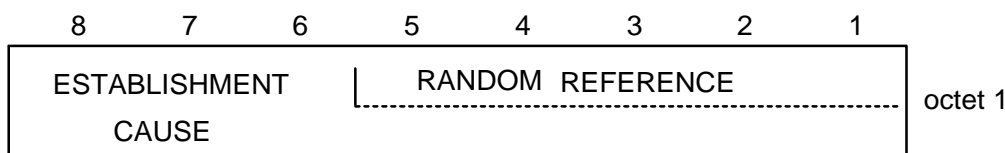
Figure 9.1.45.1/3GPP TS 44.018: UPLINK ACCESS message content
