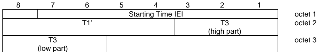
Figure 10.5.2.38.1/3GPP TS 44.018: Starting Time information element
