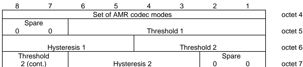
Figure 10.5.2.21aa.4/3GPP TS 44.018: Parameters for multirate speech field for the Multirate speech versions 1 & 2 when a set of three codec modes is chosen
