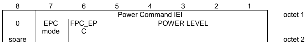
Figure 10.5.2.28.1/3GPP TS 44.018: Power Command information element
