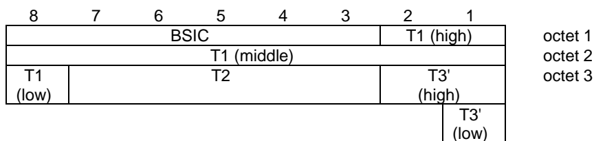
Figure 9.1.30a.1/3GPP TS 44.018: Frame synchronization information element
