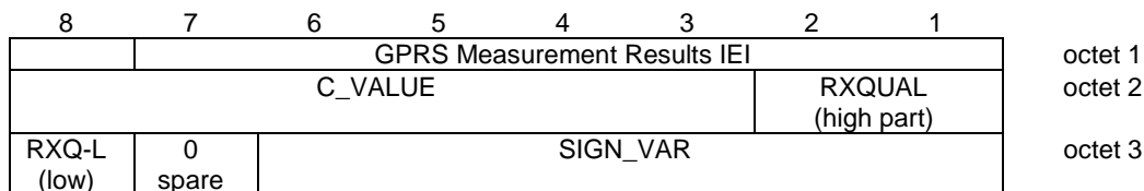
Figure 10.5.2.20a.1/3GPP TS 44.018: GPRS Measurement Results information element
