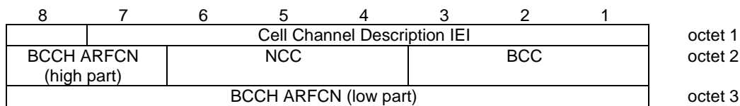
Figure 10.5.2.2.1/3GPP TS 44.018: Cell Description information element
