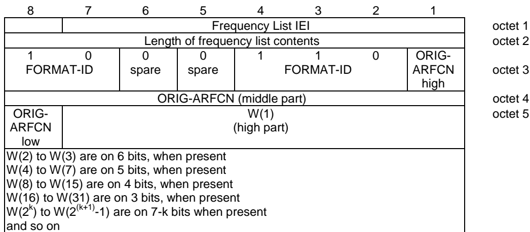
Figure 10.5.2.13.6.1/3GPP TS 44.018: Frequency List information element (Range 128 format)
