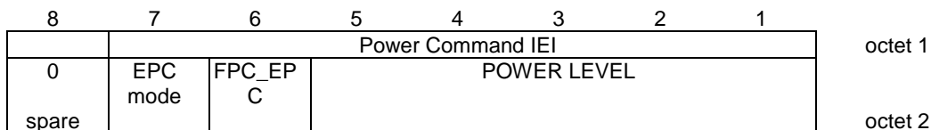
Figure 10.5.2.28.1/3GPP TS 44.018: Power Command information element
