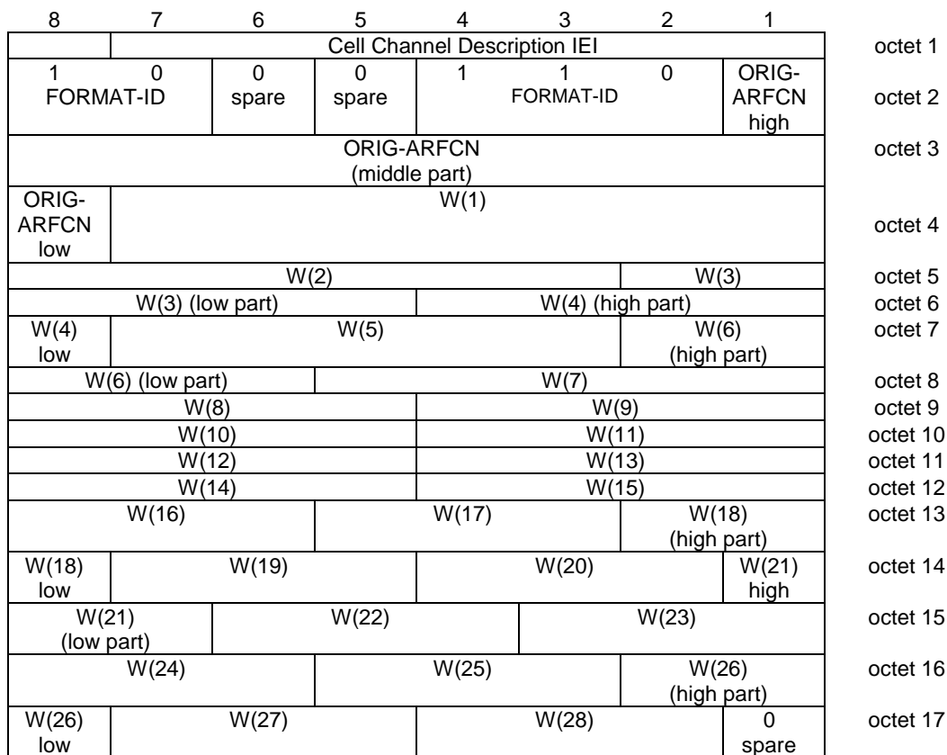
Figure 10.5.2.1b.6.1//3GPP TS 44.018: Cell Channel Description information element, range 128 format
