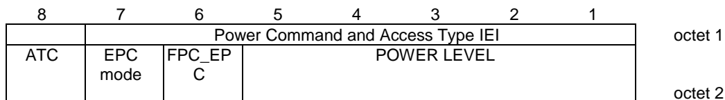
Figure 10.5.2.28a.1/3GPP TS 44.018: Power Command and access type information element
