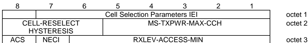
Figure 10.5.2.4.1/3GPP TS 44.018: Cell Selection Parameters information element
