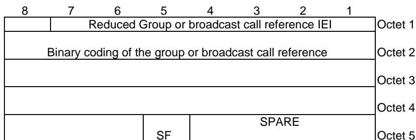
Figure 10.5.2.63.1 Reduced Group or Broadcast Call Reference
