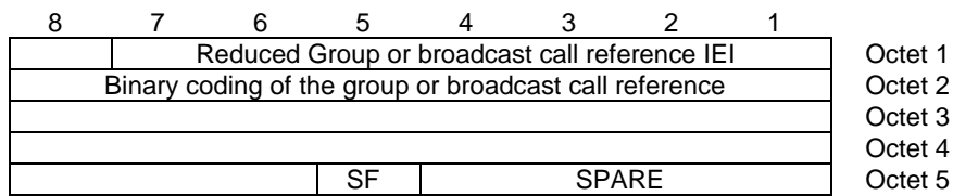
Figure 10.5.2.63.1 Reduced Group or Broadcast Call Reference
