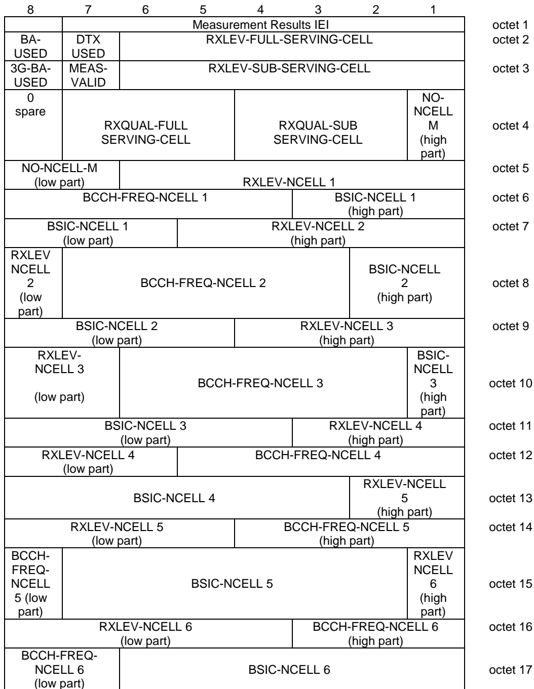
Figure 10.5.2.20.1: Measurement Results information element
