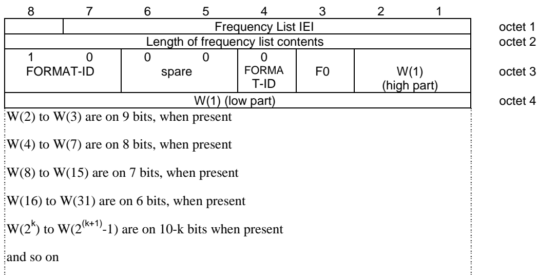
Figure 10.5.2.13.3.1: Frequency List information element (Range 1024 format)
