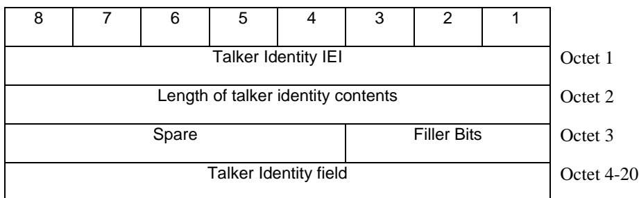
Figure 10.5.2.65.1: Talker identity information element
