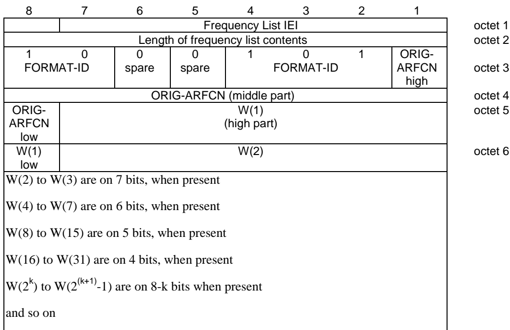
Figure 10.5.2.13.5.1: Frequency List information element (Range 256 format)
