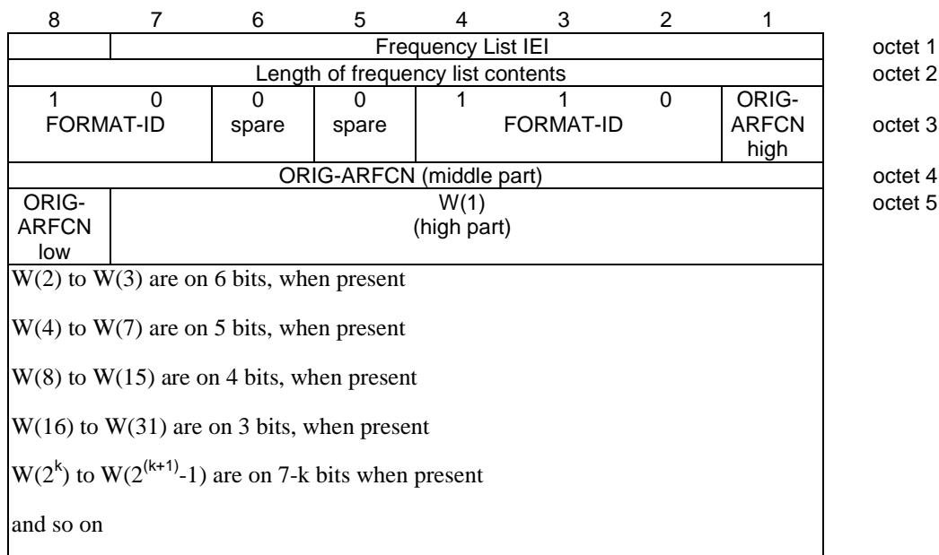
Figure 10.5.2.13.6.1: Frequency List information element (Range 128 format)
