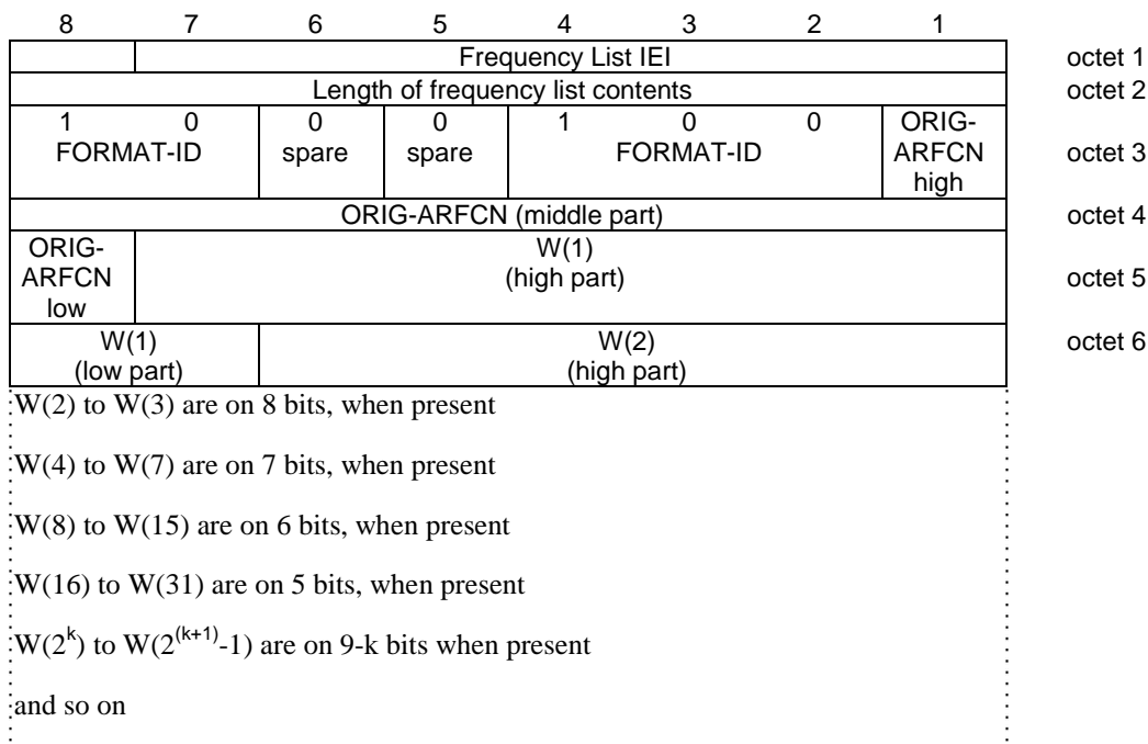
Figure 10.5.2.13.4.1: Frequency List information element (Range 512 format)
