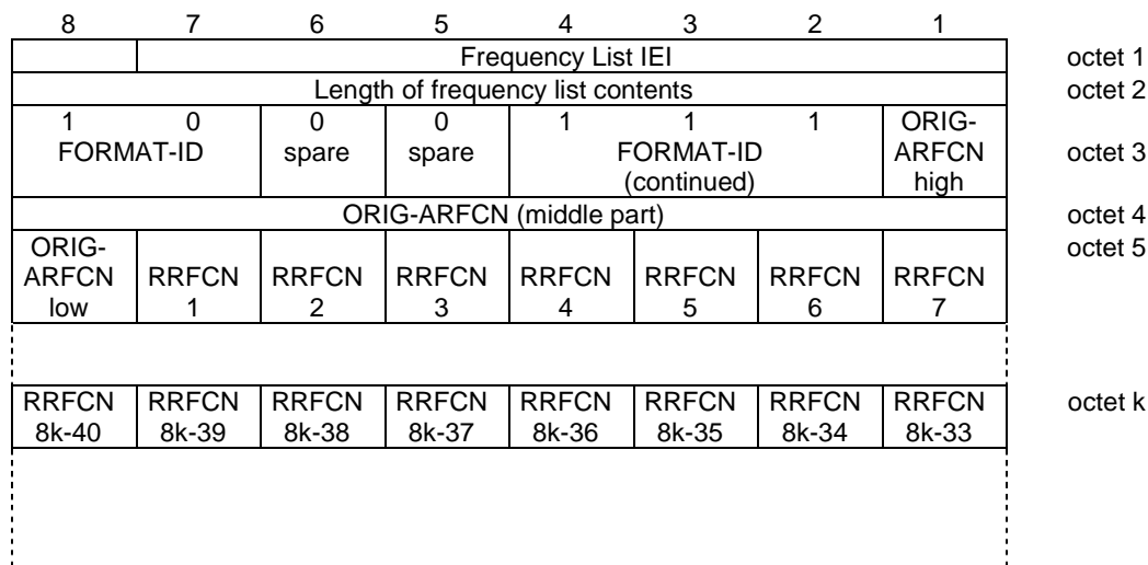
Figure 10.5.2.13.7.1: Frequency List information element, variable bit map format
