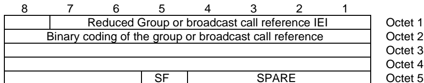
Figure 10.5.2.63.1 Reduced Group or Broadcast Call Reference
