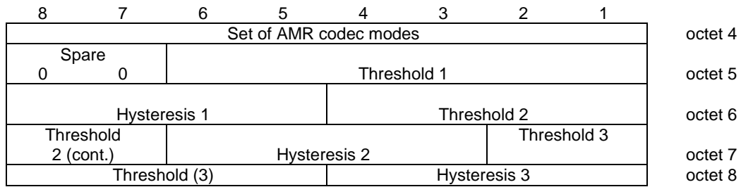
Figure 10.5.21aa.5: Parameters for multirate speech field for the Multirate speech versions 1 & 2 when a set of four modes is chosen
