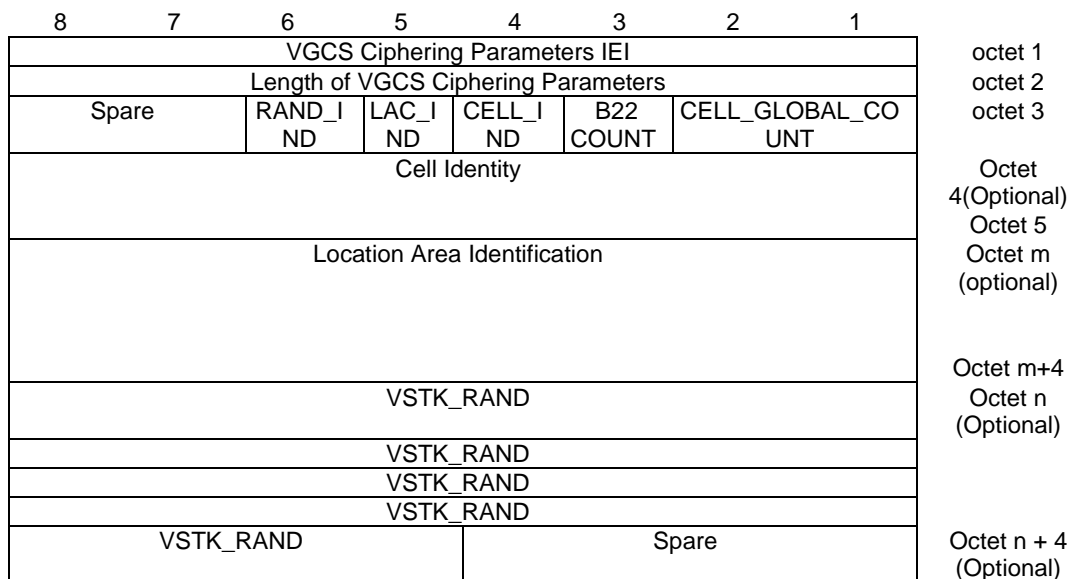
Figure 10.5.2.42b.1: VGCS Cipheryng Parameters Information Element
