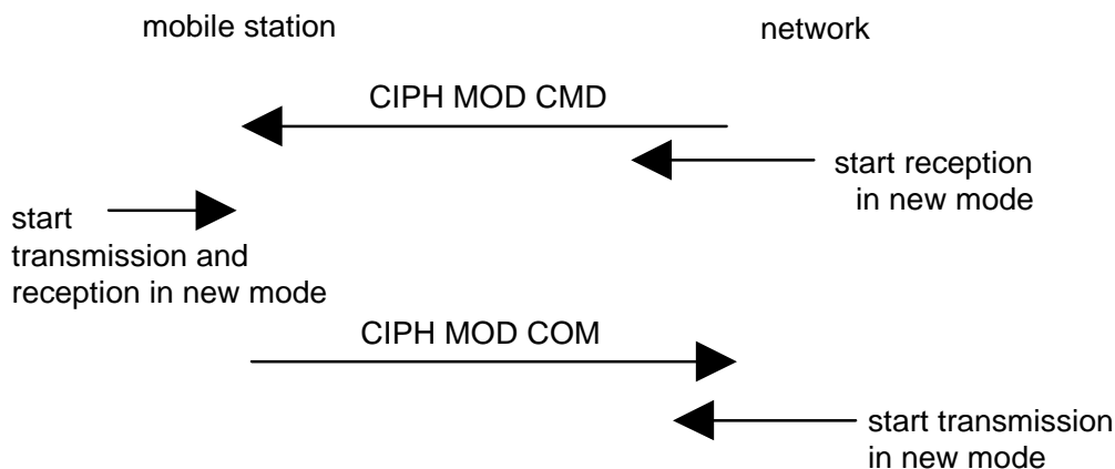
Figure 3.4.7.2.1: Cipherng mode setting sequence
