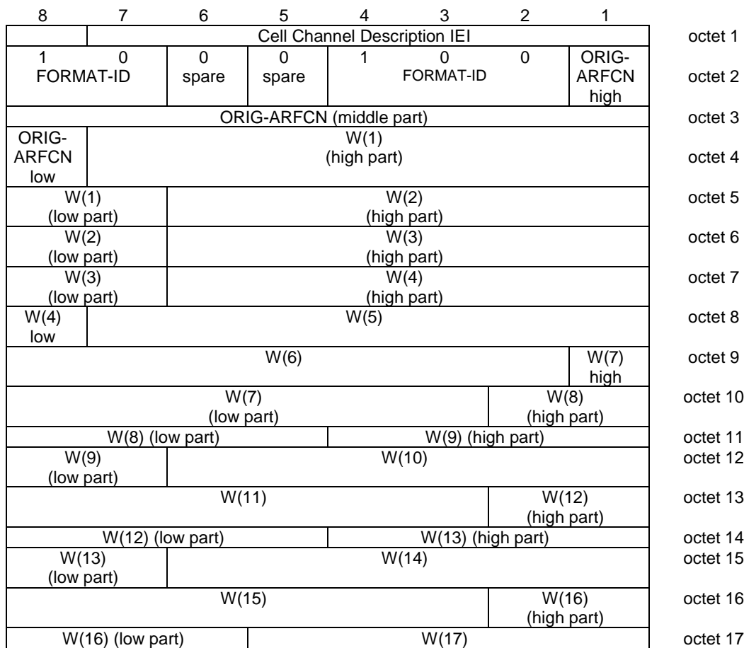
Figure 10.5.2.1b.4.1: Cell Channel Description information element (512 range format)
