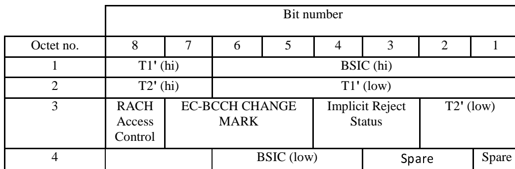
Figure 9.1.30c.1: EC-SCH INFORMATION message information elements
