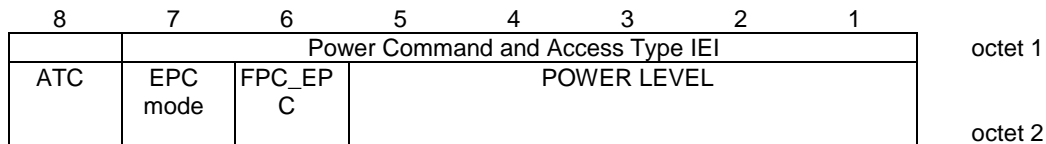
Figure 10.5.2.28a.1: Power Command and access type information element
