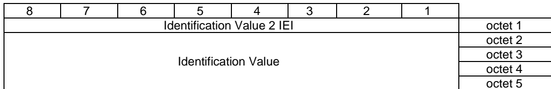
Figure 10.5.2.66.1: Token information element
