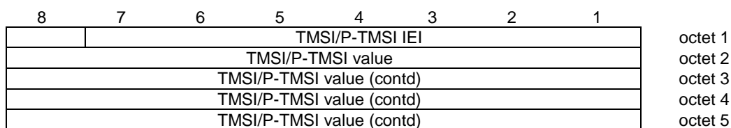
Figure 10.5.2.42.1: TMSI/P-TMSI information element
