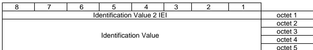
Figure 10.5.2.66.1: Token information element
