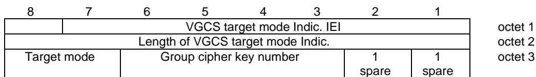
Figure 10.5.2.42a.1: VGCS target mode Indication information element
