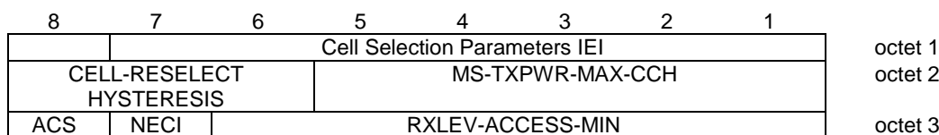
Figure 10.5.2.4.1: Cell Selection Parameters information element
