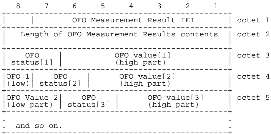
Figure 10.11/GSM 04.56 OFO Measurement Results information element
