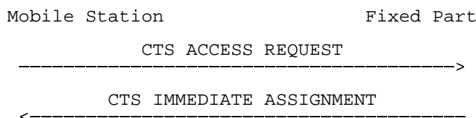
Figure 7.2/GSM 04.56: CTS immediate assignment
