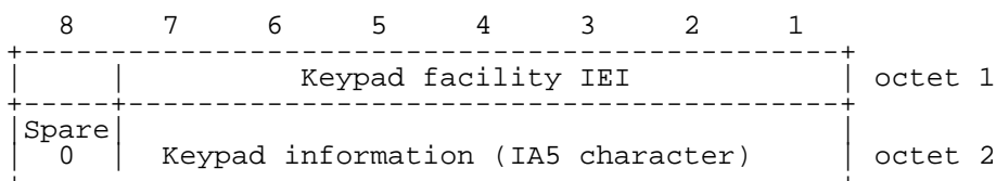
Figure 10.22/GSM 04.56: Keypad facility information element
