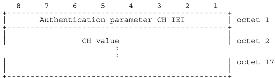
Figure 10.14/GSM 04.56: Authentication Parameter CH information element
