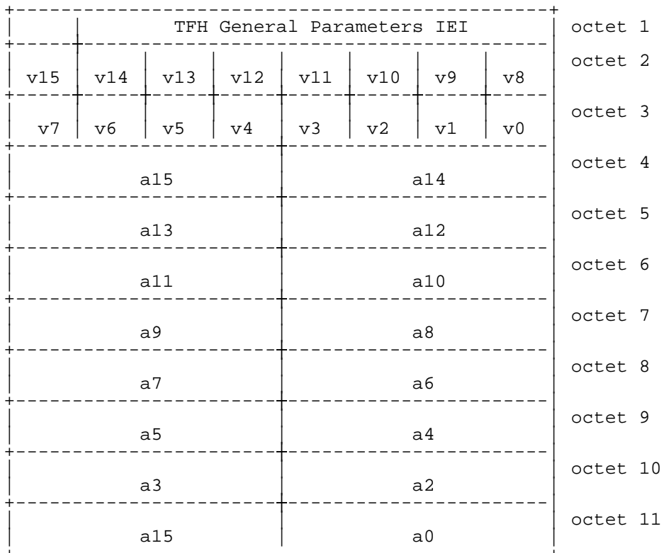
Figure 10.2/GSM 04.56: TFH General Parameters information element
