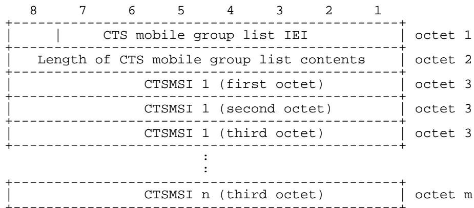
Figure 10.18/GSM 04.56: CTS mobile group list information element
