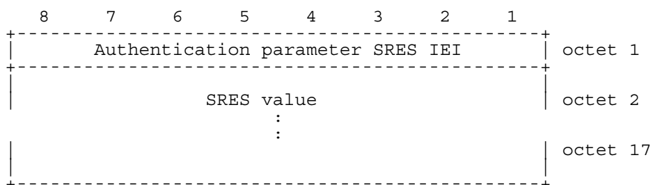
Figure 10.x/GSM 04.xx Authentication Parameter SRES information element
