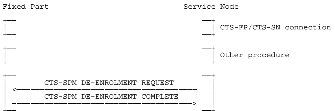
Figure 5.7/GSM 04.xx: CTS-SPM De-enrolment request
