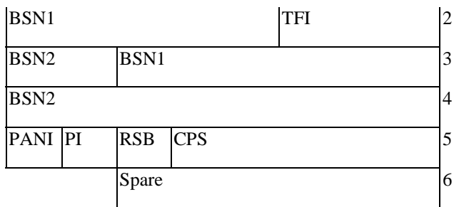
Figure 10.3a.4.1.2: EGPRS uplink RLC data block header (FANR activated) for MCS-7, MCS-8 and MCS-9.
