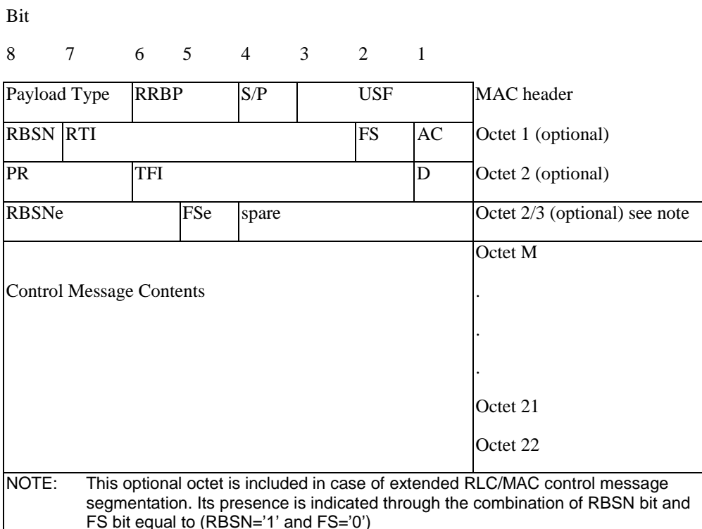
Figure 10.3.1.1: Downlink RLC/MAC control block together with its MAC header
