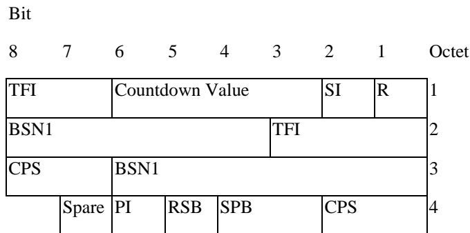
Figure 10.3a.4.3.1: EGPRS uplink RLC data block header (FANR not activated) for MCS-1, MCS-2, MCS-3 and MCS-4.
