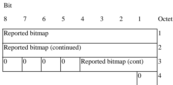
Figure 10.3a.6.1: Piggy-backed Ack/Nack field (Time-based)
