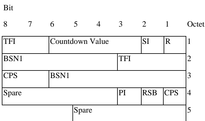
Figure 10.3a.4.2.1: EGPRS uplink RLC data block header (FANR not activated) for MCS-5 and MCS-6
