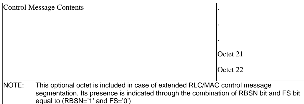
Figure 10.3.1.2: Downlink RLC/MAC control block message contents
