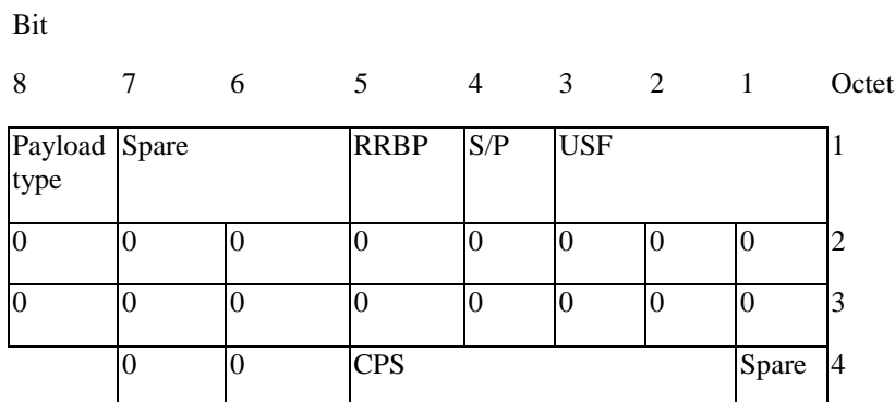
Figure 10.3a.3.3.3: Downlink RLC/MAC control block header for MCS-0.
