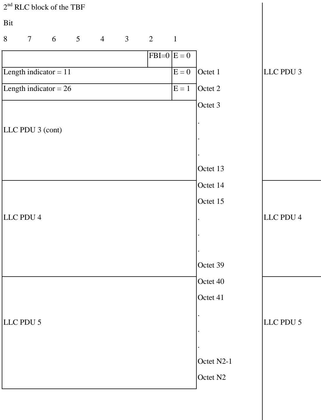
Figure B.8: Example for the case when a LLC PDU stretches over more than 2 consecutive in sequence RLC data blocks (LLC PDU 3 and LLC PDU 5).
