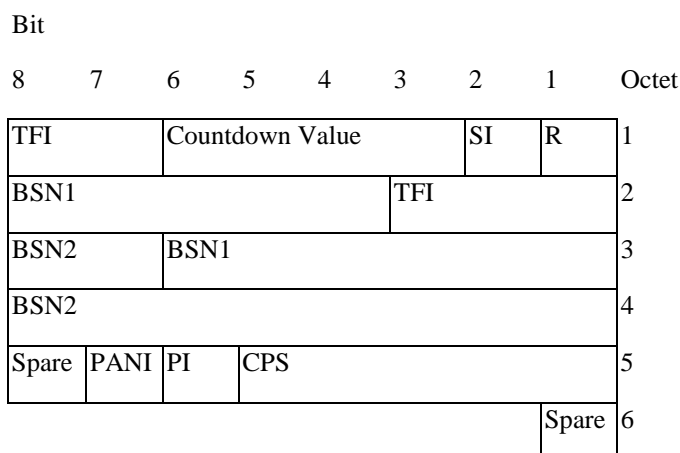
Figure 10.3a.4.4.1: Combined uplink RLC data block header for UAS-7, UAS-8 and UAS-9.
