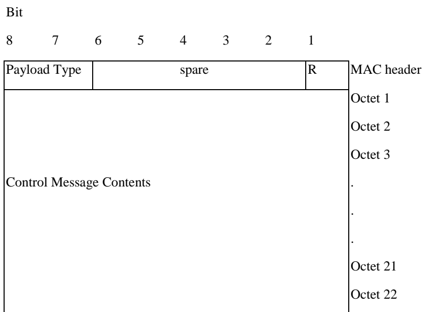
Figure 10.3.2.1: Uplink RLC/MAC control block together with its MAC header
