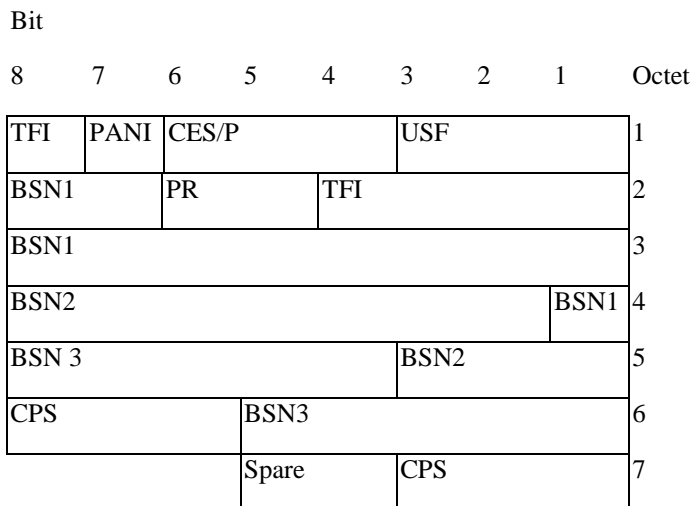
Figure 10.3a.3.8.1: Combined downlink RLC data block header for DBS-9 and DBS-10.
