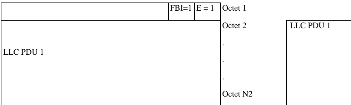
Figure B.10: Example for the case when a LLC PDU fills the RLC data block precisely.
