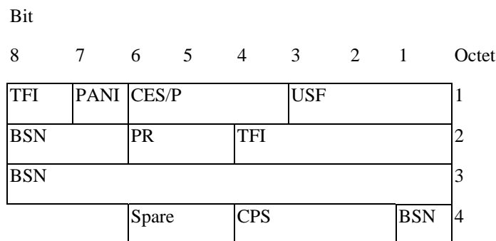
Figure 10.3a.3.6.1: Combined downlink RLC data block header for DBS-5 and DBS-6.
