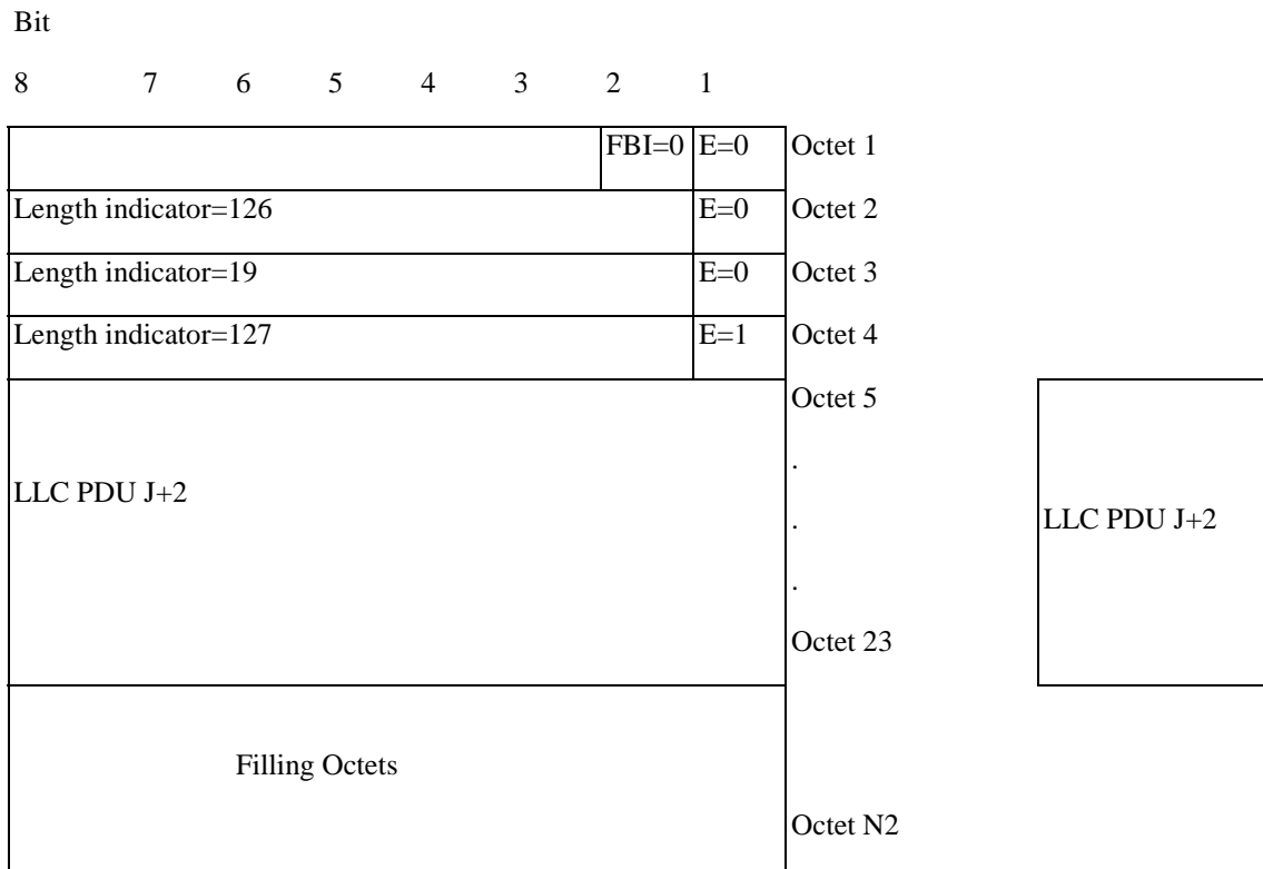
Figure B.11: Example for the case when the LLC PDU J+1 ends in the previous RLC data block and the start of the next LLC PDU J+2 is in the next RLC data block which is indicated using LI=126 as the first LI in that RLC data block.
