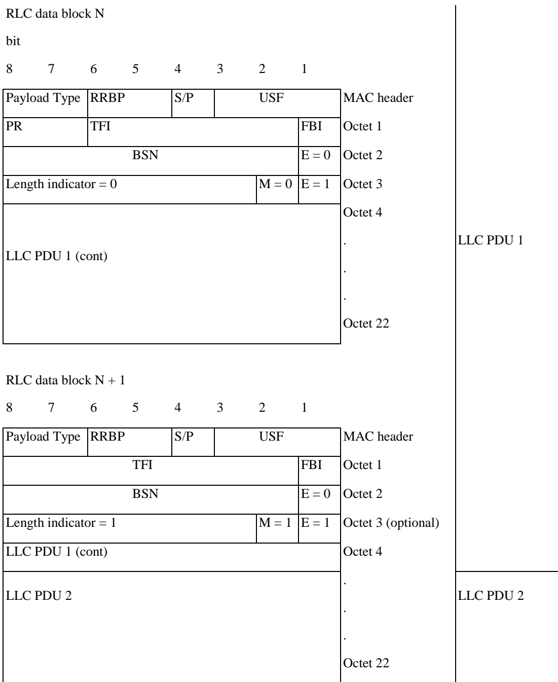
Figure B.2: Length indicator (LI) example
