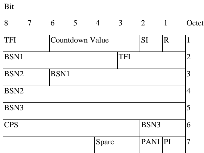
Figure 10.3a.4.5.1: Combined uplink RLC data block header for UAS-10, UAS-11.
