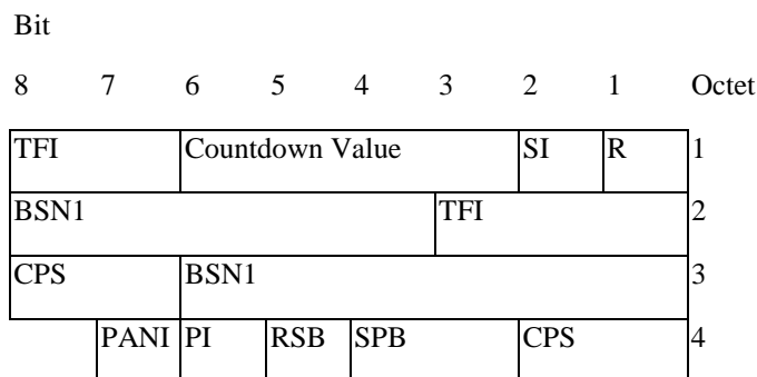
Figure 10.3a.4.3.2: EGPRS (FANR activated)/EGPRS2 uplink RLC data block header for MCS-1, MCS-2, MCS-3 and MCS-4.
