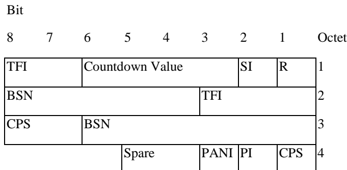
Figure 10.3a.4.6.1: Combined uplink RLC data block header for UBS-5, UBS-6.
