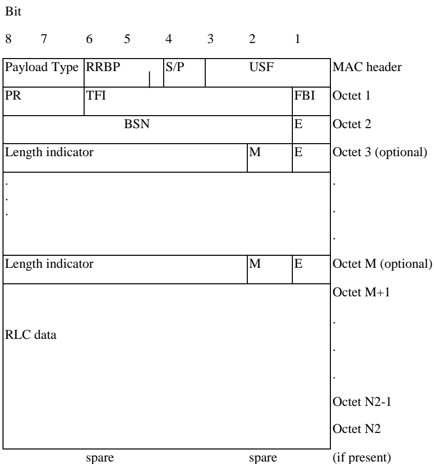
Figure 10.2.1.1: Downlink RLC data block with MAC header
