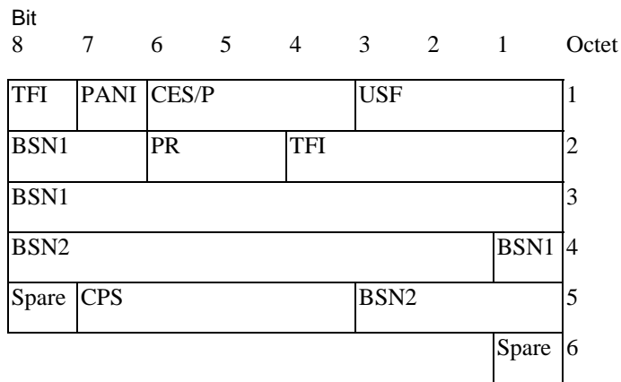
Figure 10.3a.3.7.1: Combined downlink RLC data block header for DBS-7 and DBS-8.
