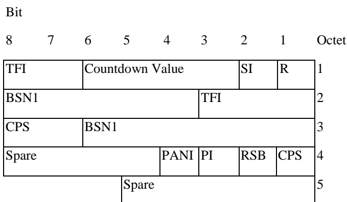
Figure 10.3a.4.2.2: EGPRS uplink RLC data block header (FANR activated) for MCS-5 and MCS-6
