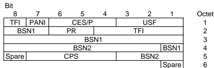
Figure 10.3a.3.7.1: Combined downlink RLC data block header for DBS-7 and DBS-8.
