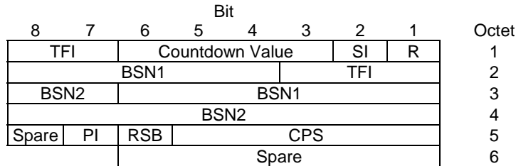
Figure 10.3a.4.1.1: EGPRS uplink RLC data block header (FANR not activated) for MCS-7, MCS-8 and MCS-9.
