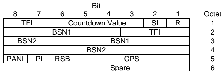
Figure 10.3a.4.1.2: EGPRS uplink RLC data block header (FANR activated) for MCS-7, MCS-8 and MCS-9.
