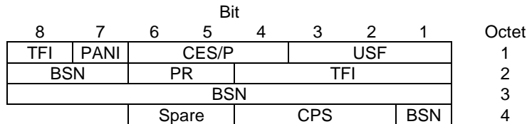
Figure 10.3a.3.6.1: Combined downlink RLC data block header for DBS-5 and DBS-6.
