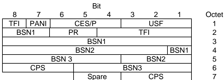
Figure 10.3a.3.8.1: Combined downlink RLC data block header for DBS-9 and DBS-10.
