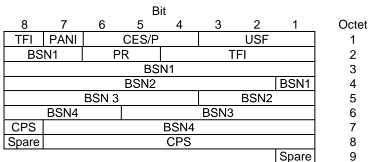
Figure 10.3a.3.9.1: Combined downlink RLC data block header for DBS-11 and DBS-12.
