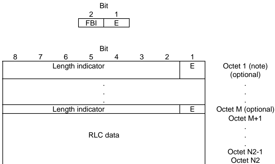
Figure 10.3a.1.1: EGPRS downlink RLC data block
