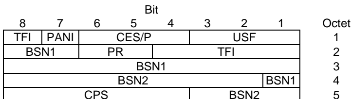
Figure 10.3a.3.1.2: EGPRS (FANR activated) / EGPRS2 downlink RLC data block header for MCS-7, MCS-8 and MCS-9.
