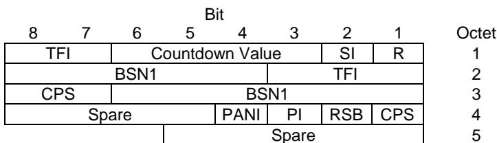
Figure 10.3a.4.2.2: EGPRS uplink RLC data block header (FANR activated) for MCS-5 and MCS-6
