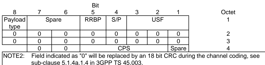
Figure 10.3a.3.3.3: Downlink RLC/MAC control block header for MCS-0.
