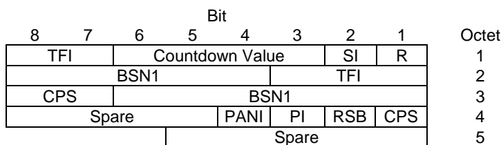
Figure 10.3a.4.2.2: EGPRS (FANR activated) / EGPRS2 uplink RLC data block header
