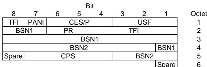
Figure 10.3a.3.4.1: Combined downlink RLC data block header for DAS-8 and DAS-9.
