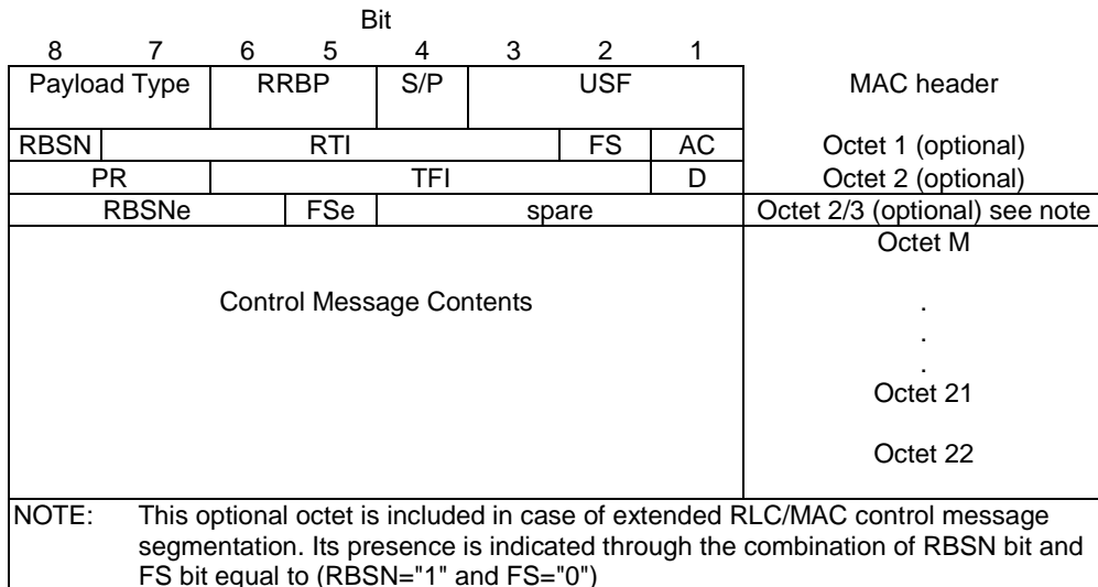
Figure 10.3.1.1: Downlink RLC/MAC control block together with its MAC header
