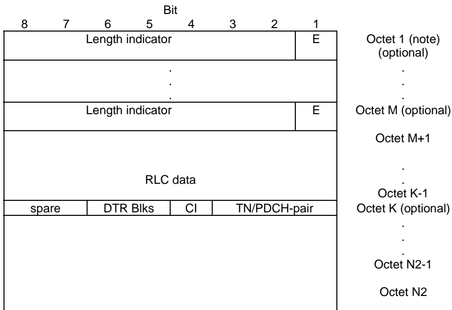
Figure 10.3a.1.1: EGPRS downlink RLC data block
