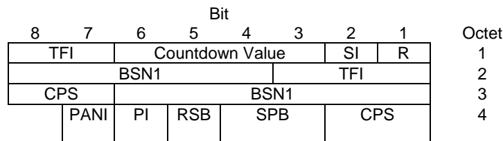
Figure 10.3a.4.3.2: EGPRS (FANR activated)/EGPRS2 uplink RLC data block header for MCS-1, MCS-2, MCS-3 and MCS-4
