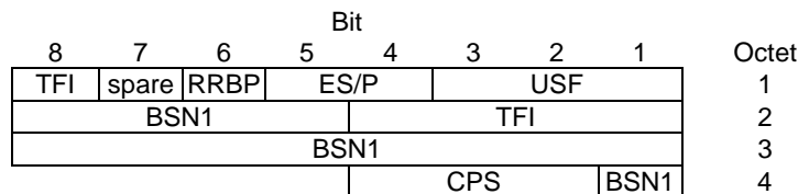
Figure 10.3a.3.2.3: DLMC EGPRS downlink RLC data block header (FANR not activated) for MCS-5 and MCS-6
