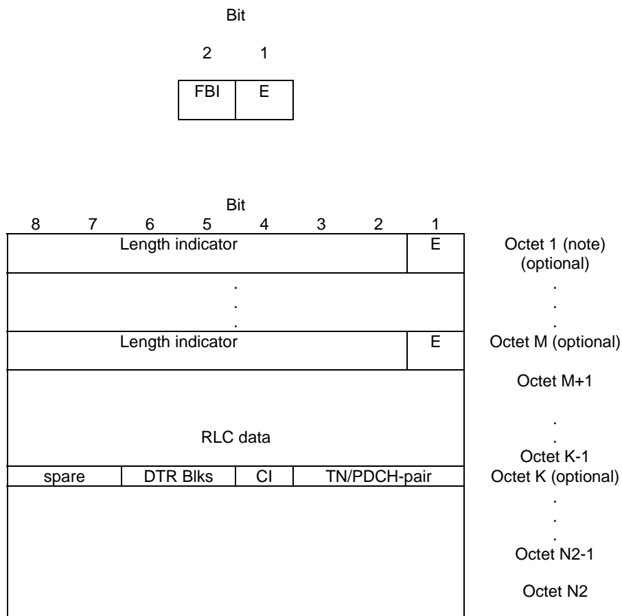
Figure 10.3a.1.1: EGPRS downlink RLC data block
