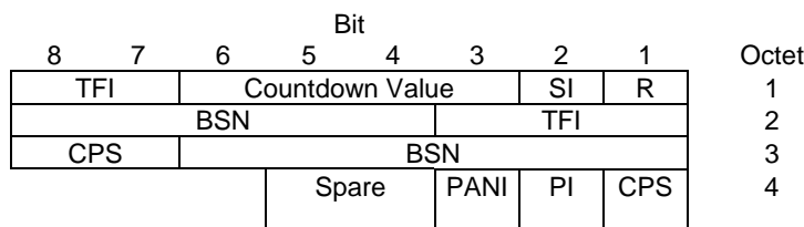
Figure 10.3a.4.6.1: Combined uplink RLC data block header for UBS-5, UBS-6.
