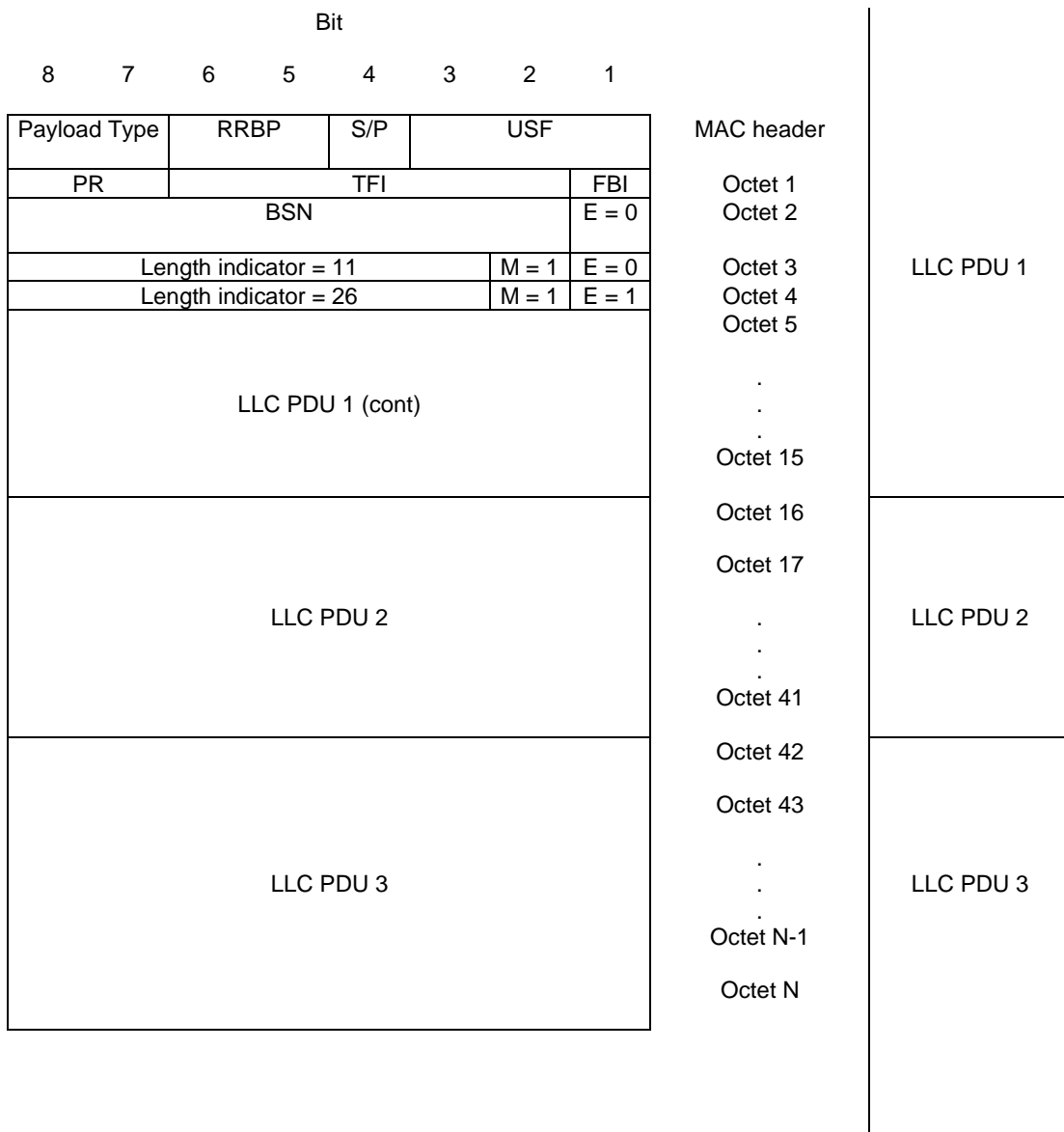
Figure B.1: Length indicator (LI) example
