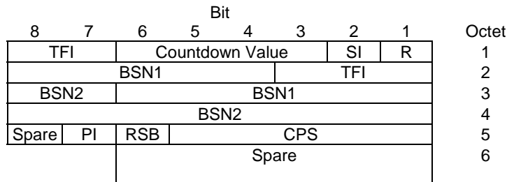
Figure 10.3a.4.1.1: EGPRS uplink RLC data block header (FANR not activated) for MCS-7, MCS-8 and MCS-9.
