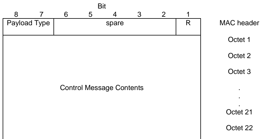
Figure 10.3.2.1: Uplink RLC/MAC control block together with its MAC header
