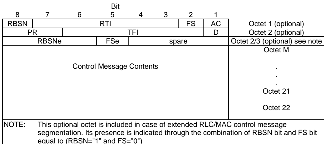
Figure 10.3.1.2: Downlink RLC/MAC control block message contents
