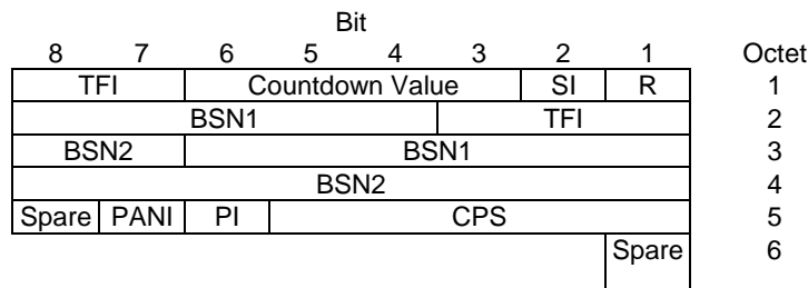
Figure 10.3a.4.4.1: Combined uplink RLC data block header for UAS-7, UAS-8 and UAS-9.
