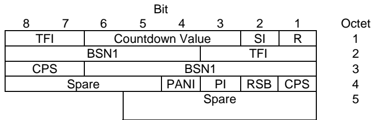
Figure 10.3a.4.2.2: EGPRS (FANR activated) / EGPRS2 uplink RLC data block header for MCS-5 and MCS-6
