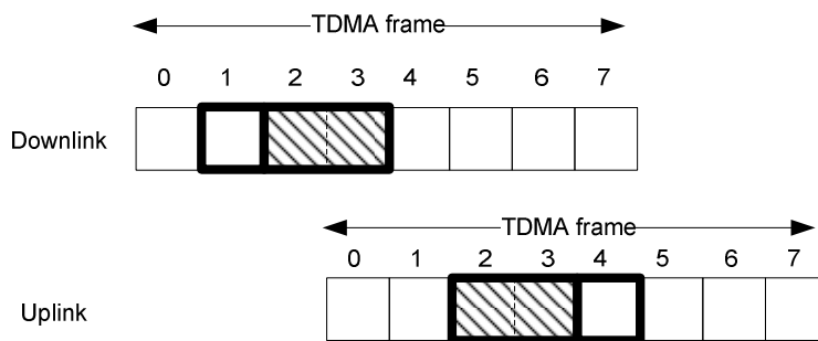
Figure M.2: Valid MTTI assignment (1 uplink TBF & 1 downlink TBF)
