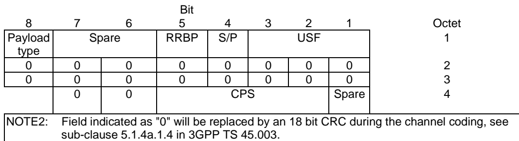
Figure 10.3a.3.3.3: Downlink RLC/MAC control block header for MCS-0.
