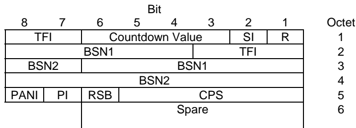
Figure 10.3a.4.1.2: EGPRS uplink RLC data block header (FANR activated) for MCS-7, MCS-8 and MCS-9.
