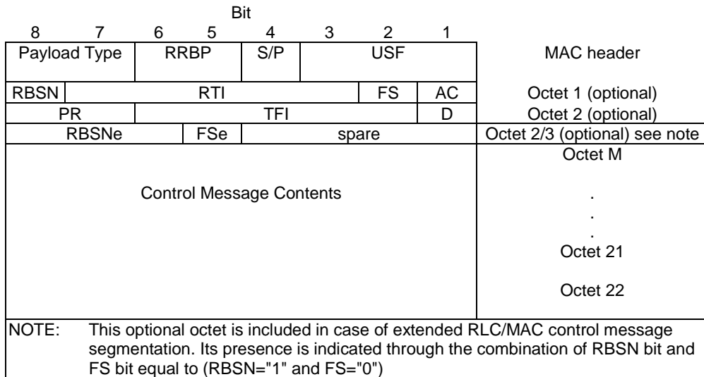
Figure 10.3.1.1: Downlink RLC/MAC control block together with its MAC header
