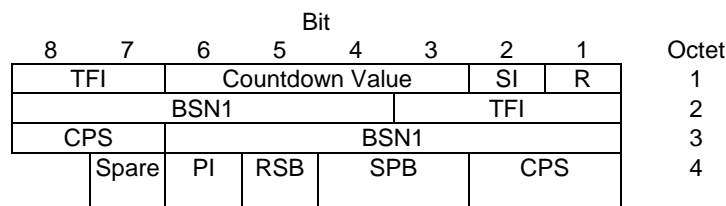
Figure 10.3a.4.3.1: EGPRS uplink RLC data block header (FANR not activated) for MCS-1, MCS-2, MCS-3 and MCS-4
