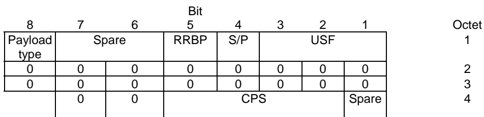
Figure 10.3a.3.3.3: Downlink RLC/MAC control block header for MCS-0.
