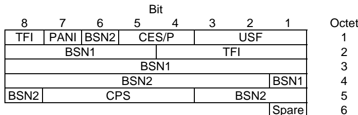
Figure 10.3a.3.4.2: DLMC Combined downlink RLC data block header for DAS-8 and DAS-9.
