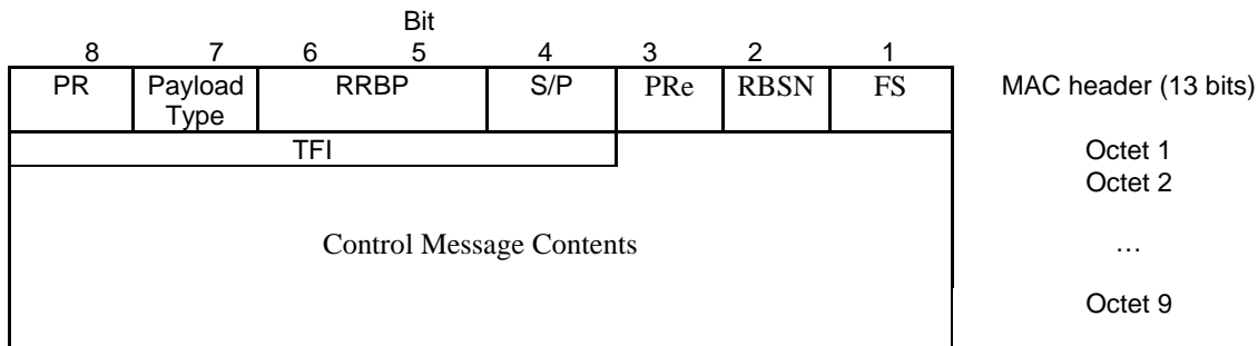
Figure 10.3.1.3.2: EC-GSM-IoT Downlink RLC/MAC control block together with its extended MAC header when Payload Type is set to 1
