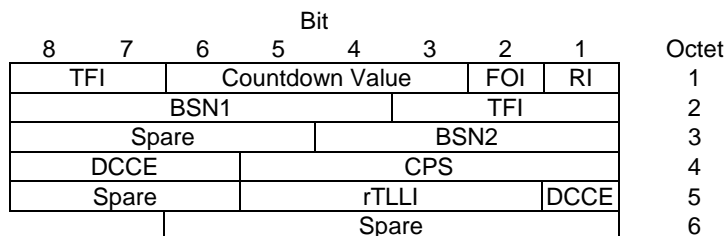
Figure 10.3a.4.1.3: EC-GSM-IoT uplink RLC data block header for MCS-7, MCS-8 and MCS-9.
